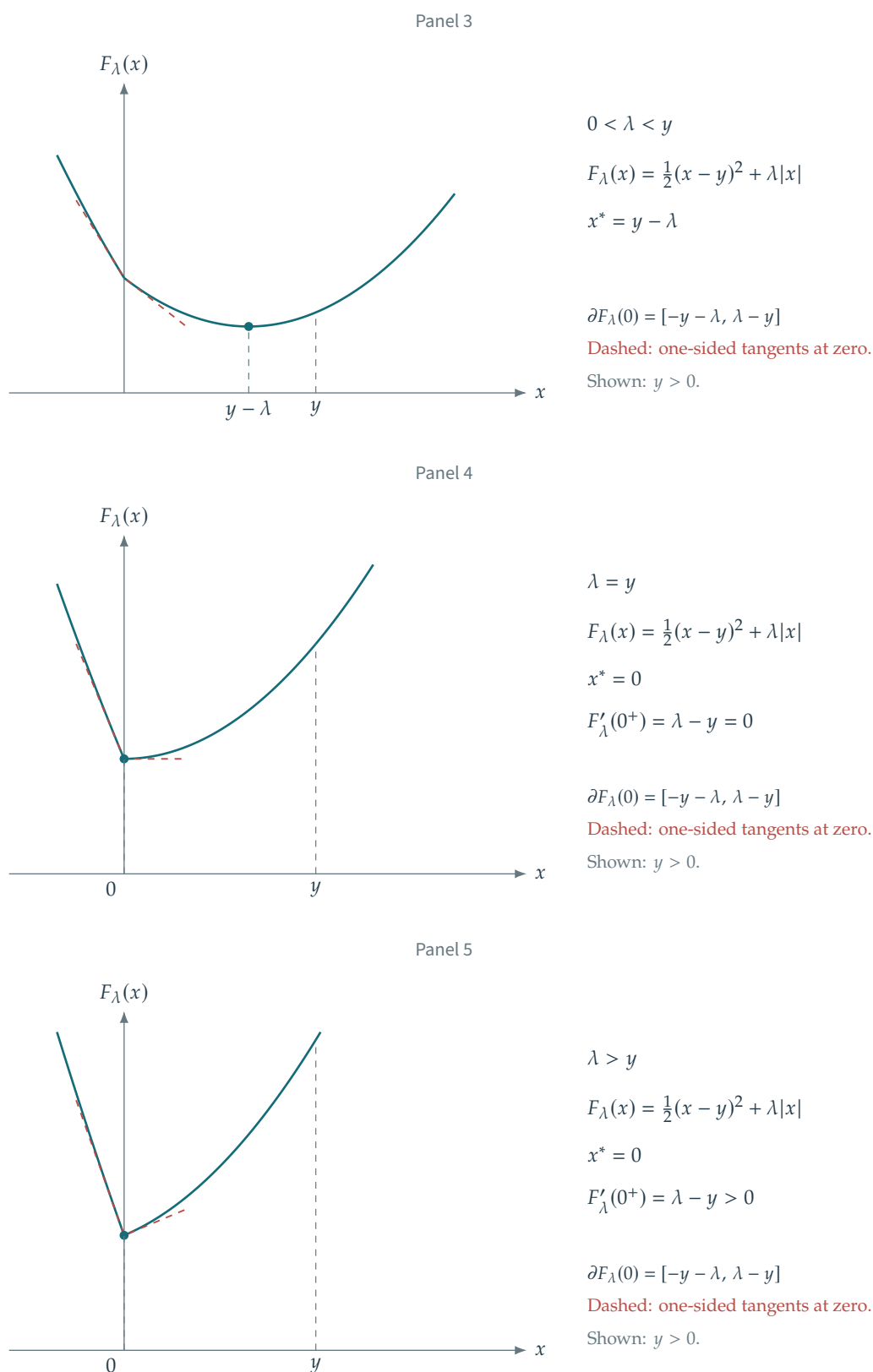
Figure 10.3 (continued). Panel 1: the objective \|\cdot - y\|^2 + T^2\|\cdot\|_0 . Panels 2–5: the scalar objective F(x) \stackrel{\text{def}}{=} \frac{1}{2}|x - y|^2 + \lambda|x| for increasing \lambda .
