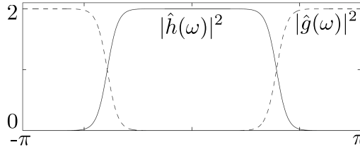
Figure 4.25. Complementarity of low-pass and high-pass filters h and g satisfying (C_3) .
