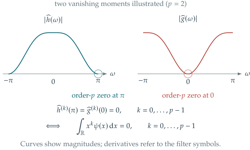
Figure 4.26. Vanishing moments correspond to vanishing derivatives of the Fourier transform.
