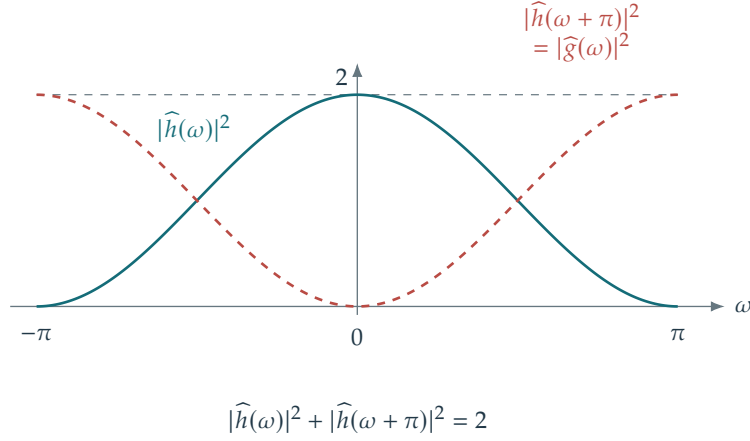
Figure 4.24. Constraints on low-pass and high-pass filters.
