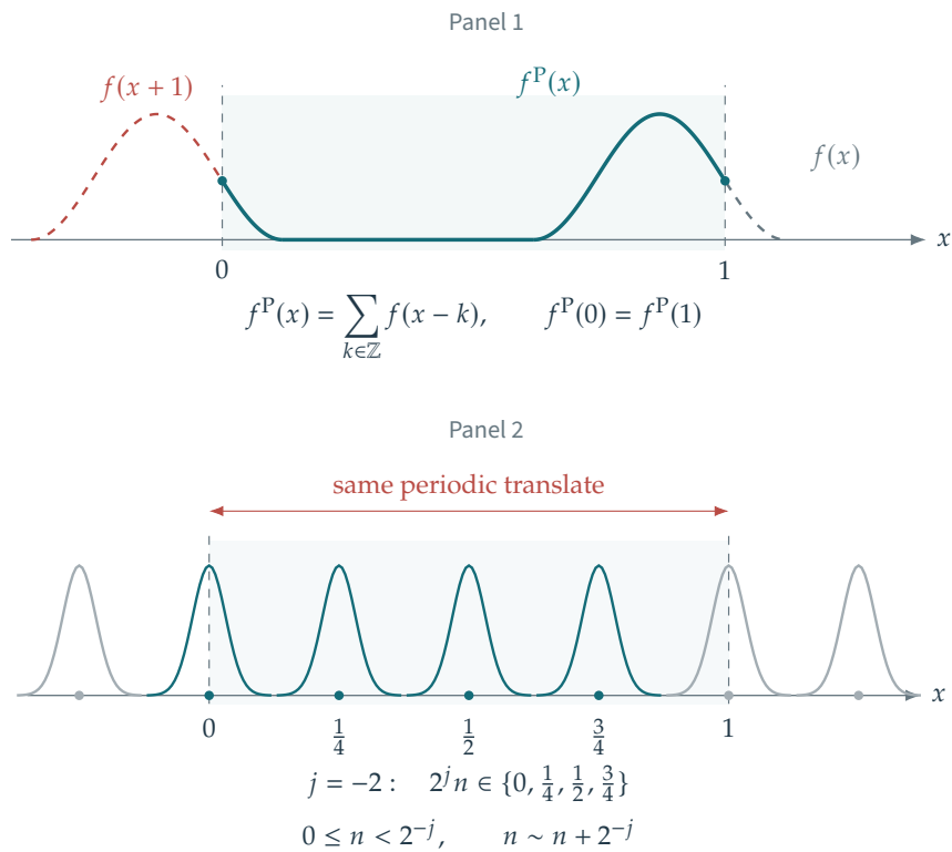
Figure 4.7. Periodized basis functions. Only the translations 0 \leq n < 2^{-j} are distinct, and j_0 = 0 is a common choice of coarsest scale.
