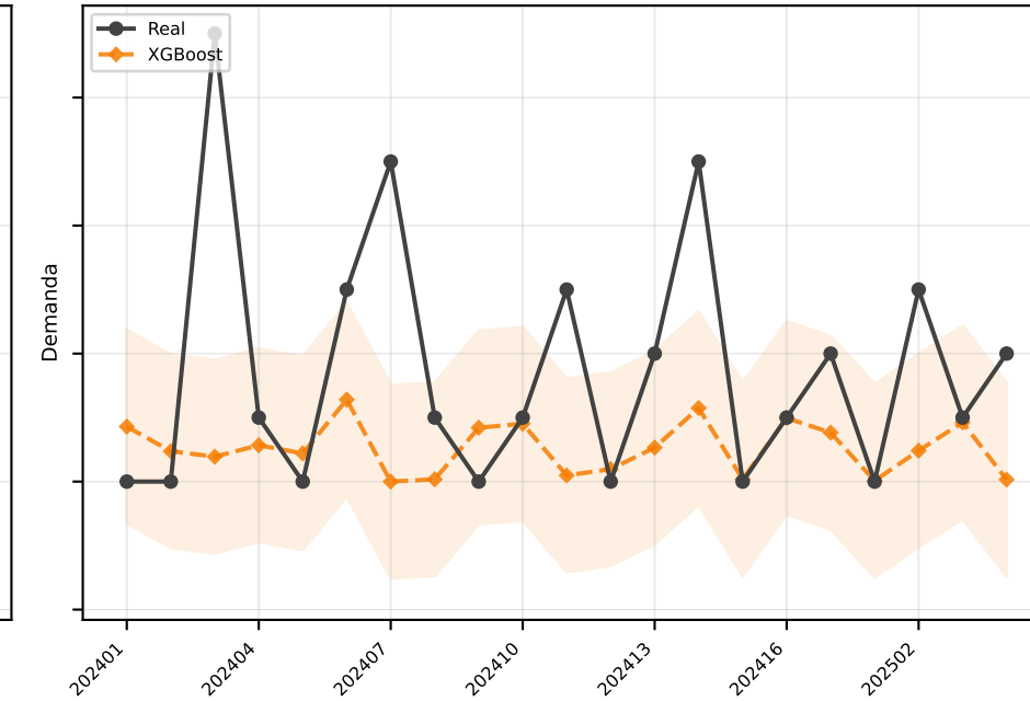
XGBoost MAE=1.5
