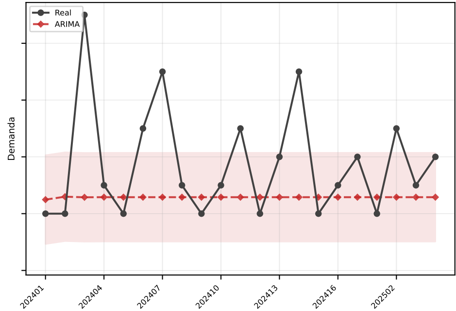
ARIMA MAE=1.6
