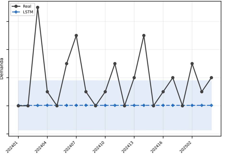
LSTM MAE=1.8
