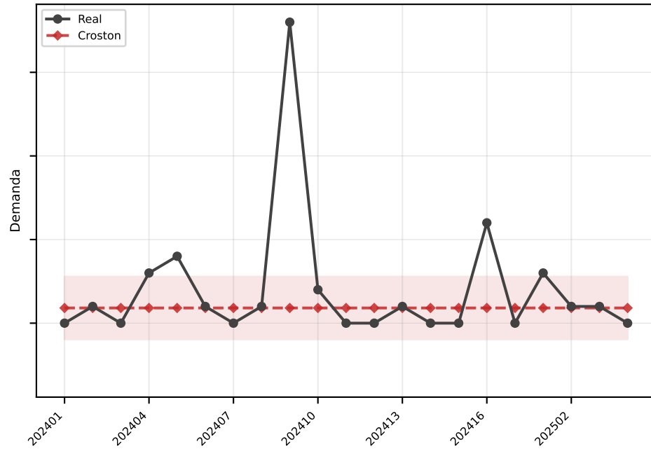
Croston MAE=1.9
