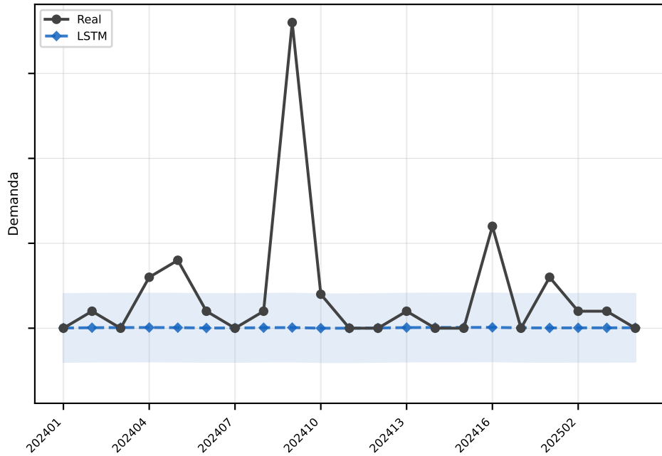
LSTM MAE=2.0
