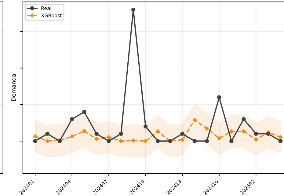
XGBoost MAE=2.2
