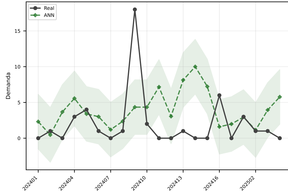
ANN MAE=3.8
