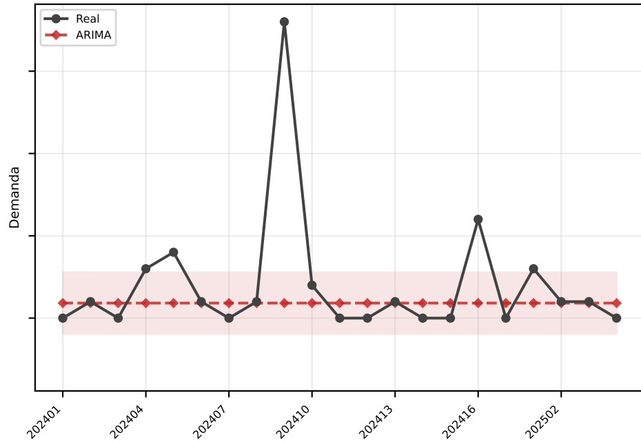
ARIMA MAE=1.9
