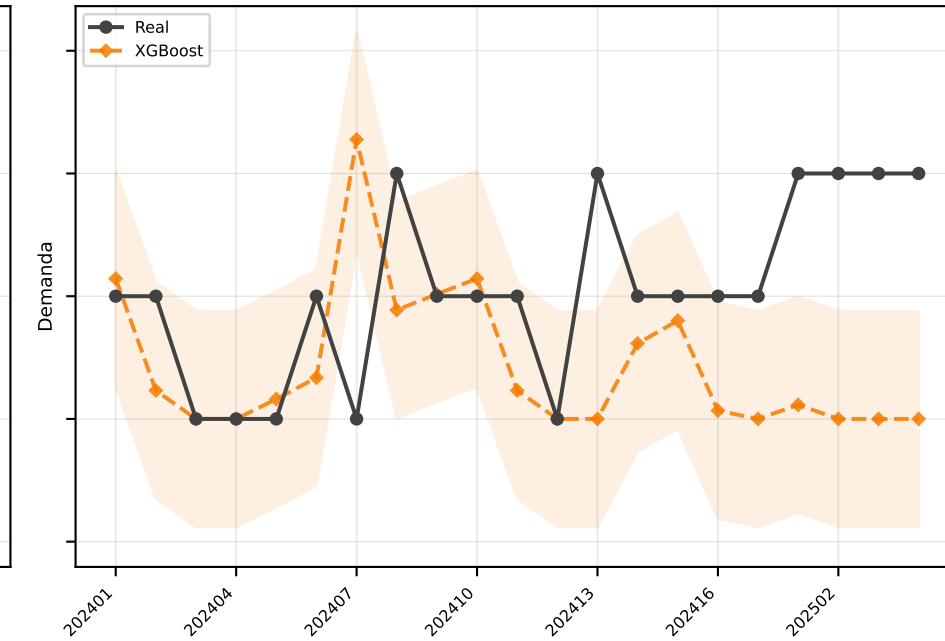
XGBoost MAE=0.9
