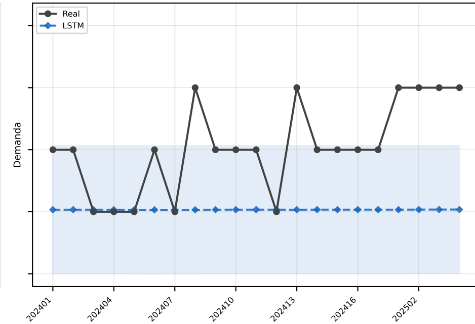
LSTM MAE=1.0
