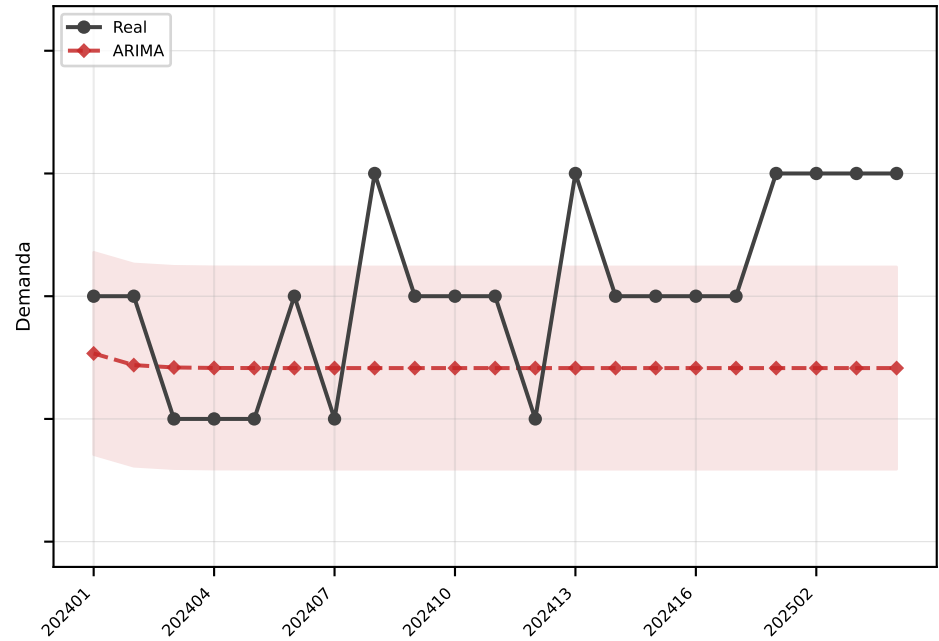
ARIMA MAE=0.8
