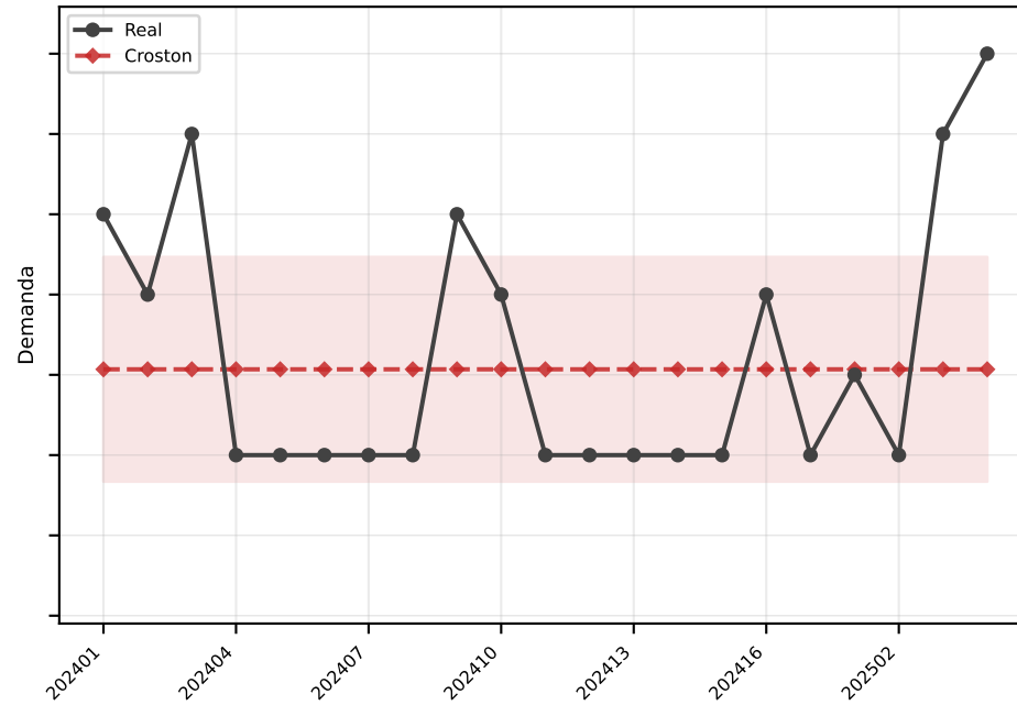
Croston MAE=1.4
