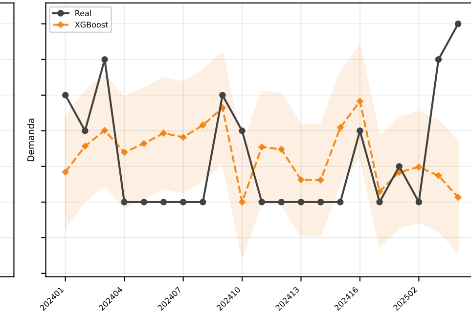
XGBoost MAE=1.6
