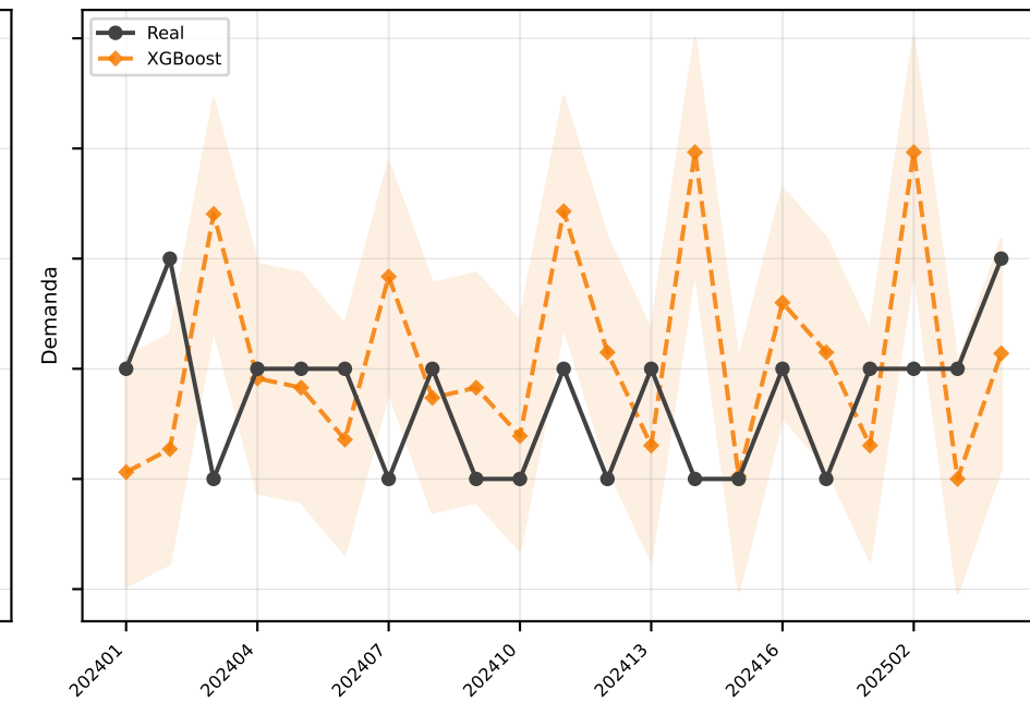
XGBoost MAE=1.0
