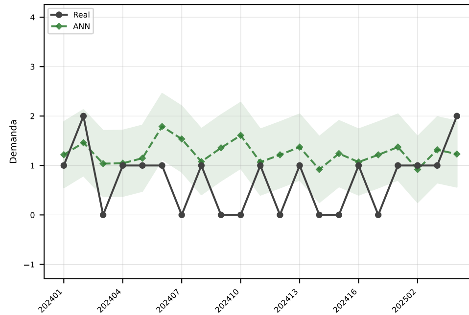
ANN MAE=0.7
