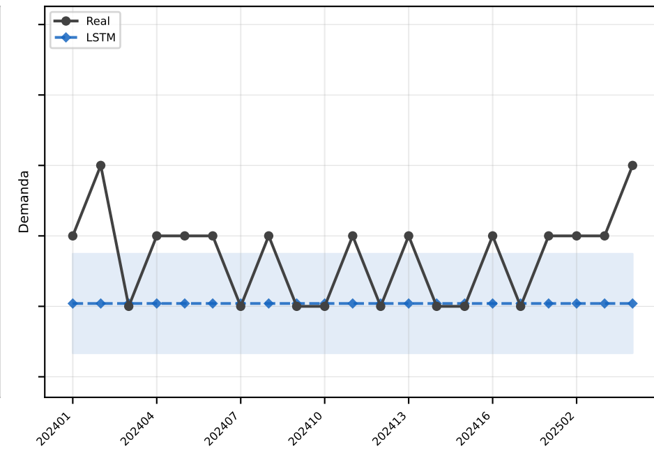
LSTM MAE=0.7
