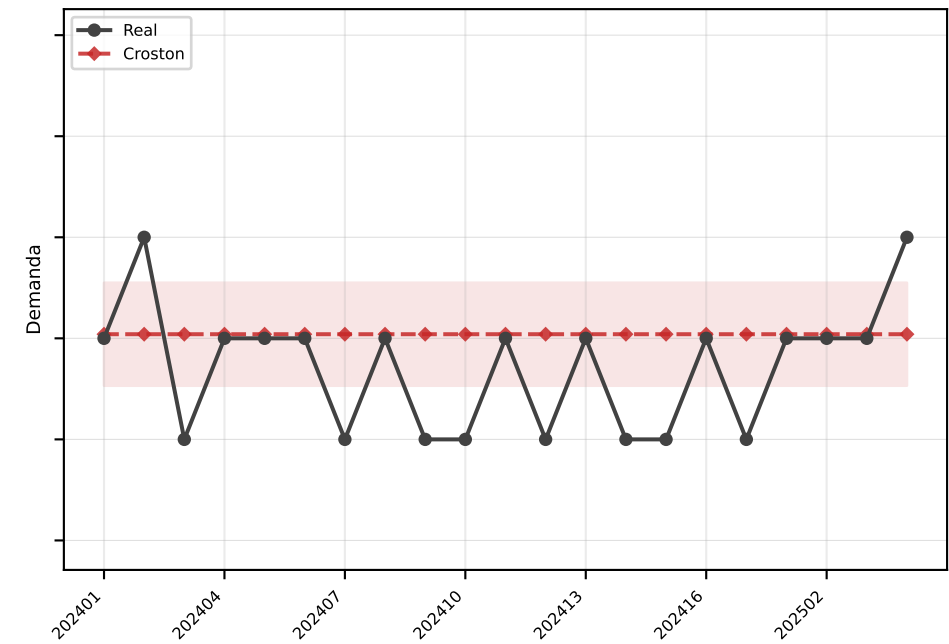
Croston MAE=0.5
