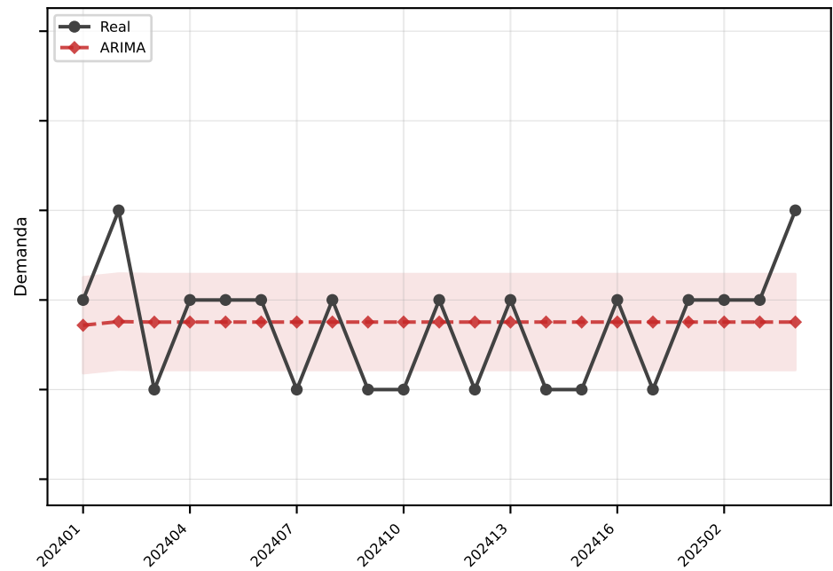
ARIMA MAE=0.5
