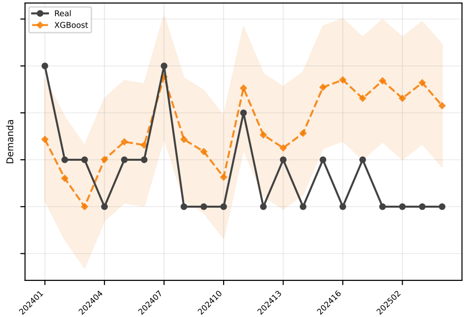
XGBoost MAE=1.3
