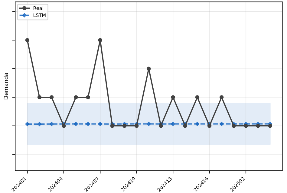
LSTM MAE=0.7
