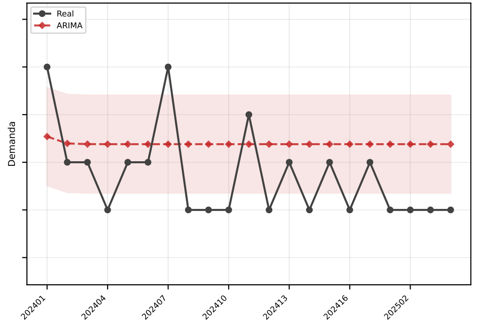
ARIMA MAE=1.0
