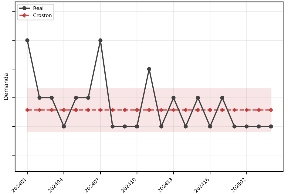
Croston MAE=0.7
