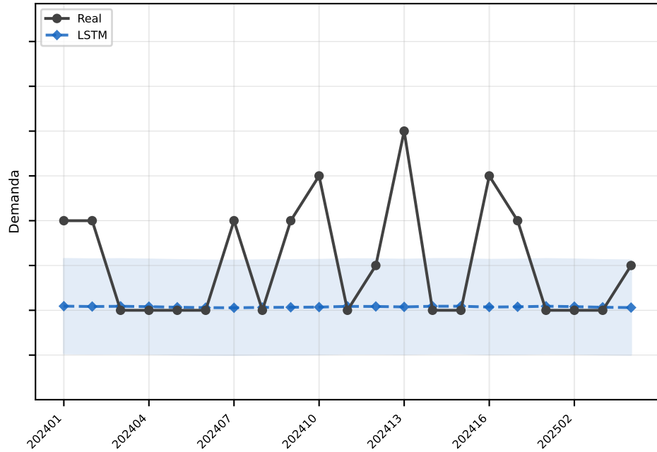
LSTM MAE=1.1
