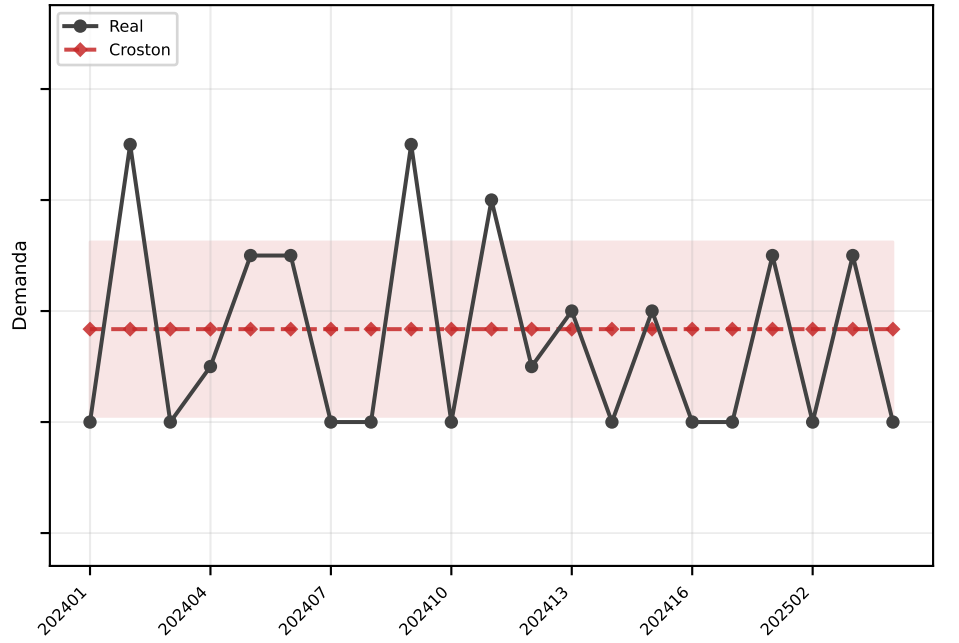
Croston MAE=1.6
