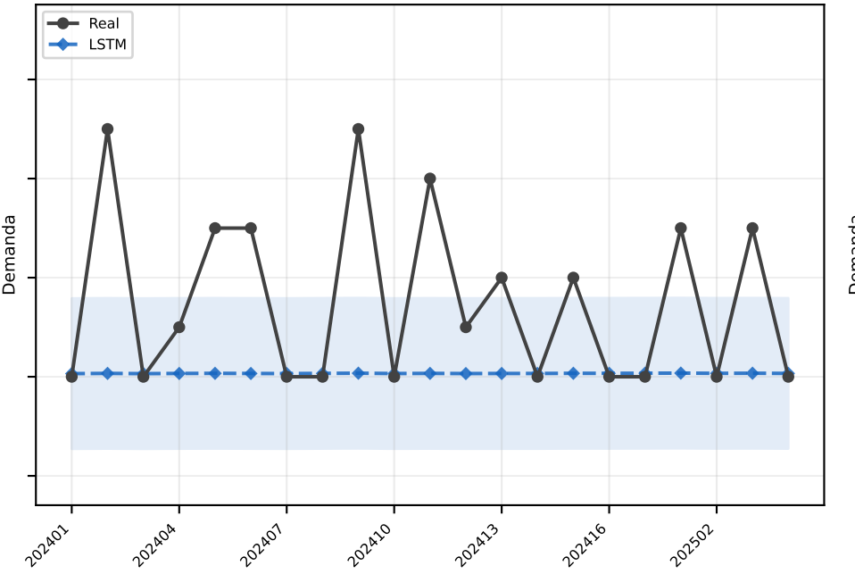
LSTM MAE=1.5
