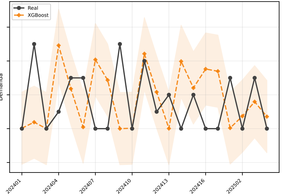
XGBoost MAE=2.1
