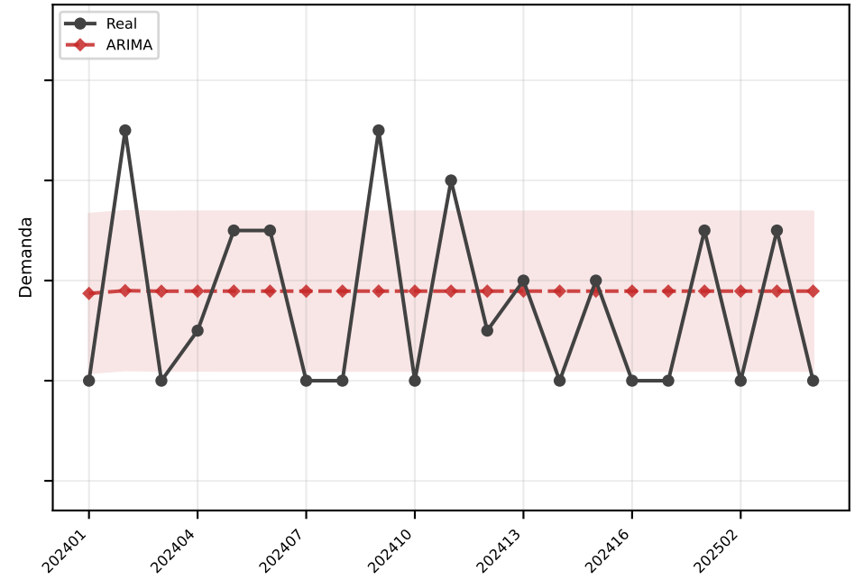
ARIMA MAE=1.6
