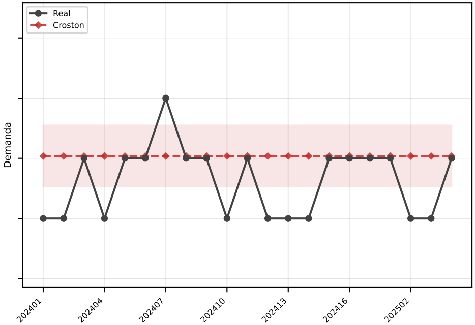
Croston MAE=0.5
