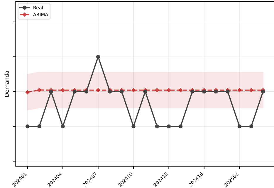
ARIMA MAE=0.5
