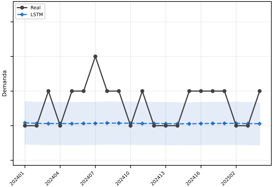
LSTM MAE=0.6
