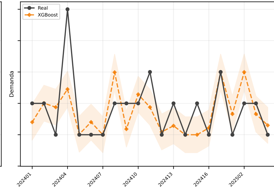
XGBoost MAE=0.6
