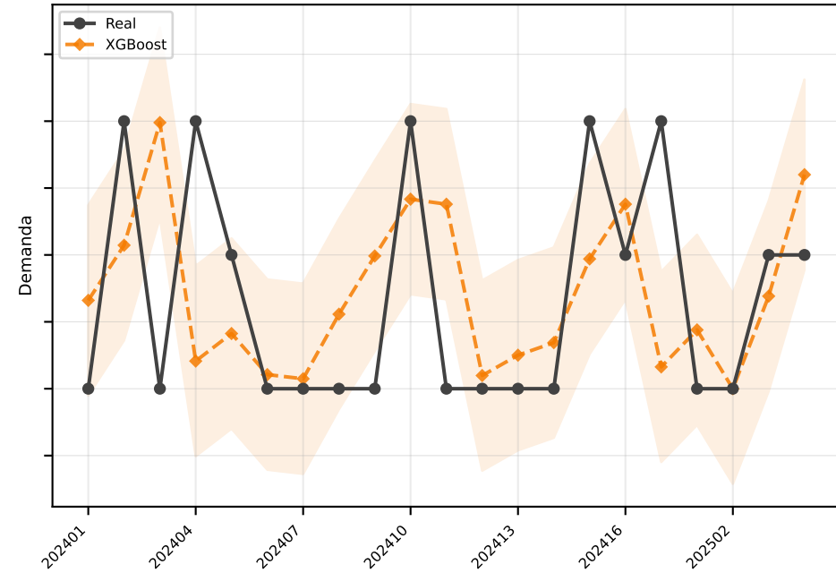
XGBoost MAE=0.7
