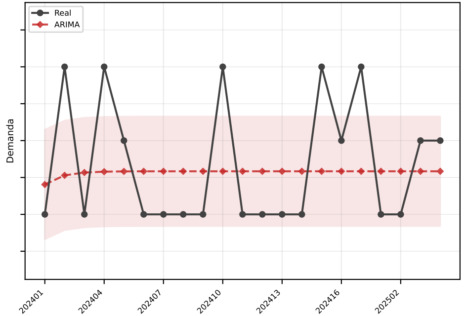
ARIMA MAE=0.7
