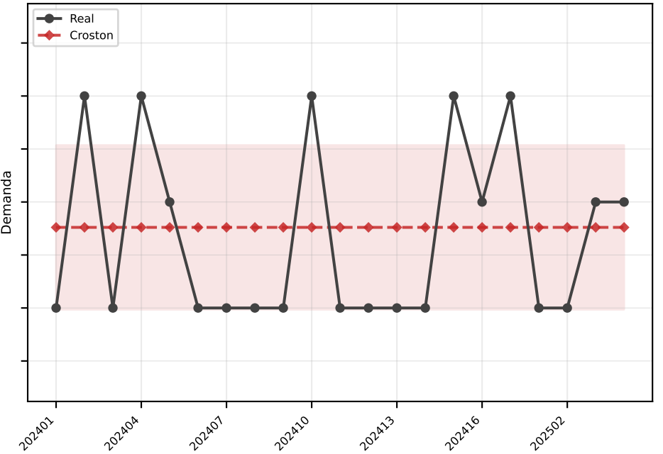
Croston MAE=0.8
