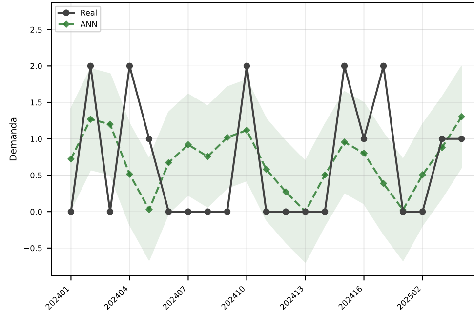
ANN MAE=0.7
