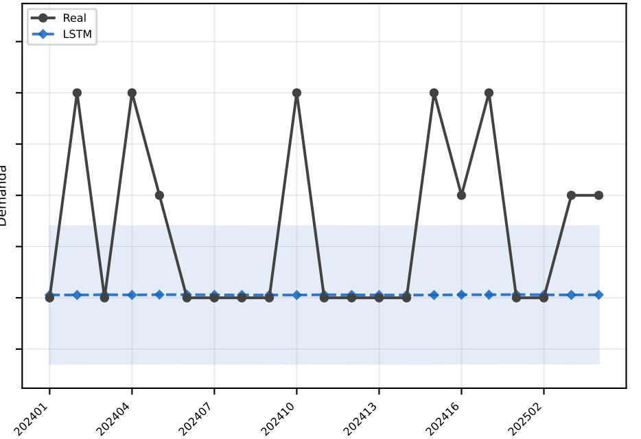
LSTM MAE=0.7
