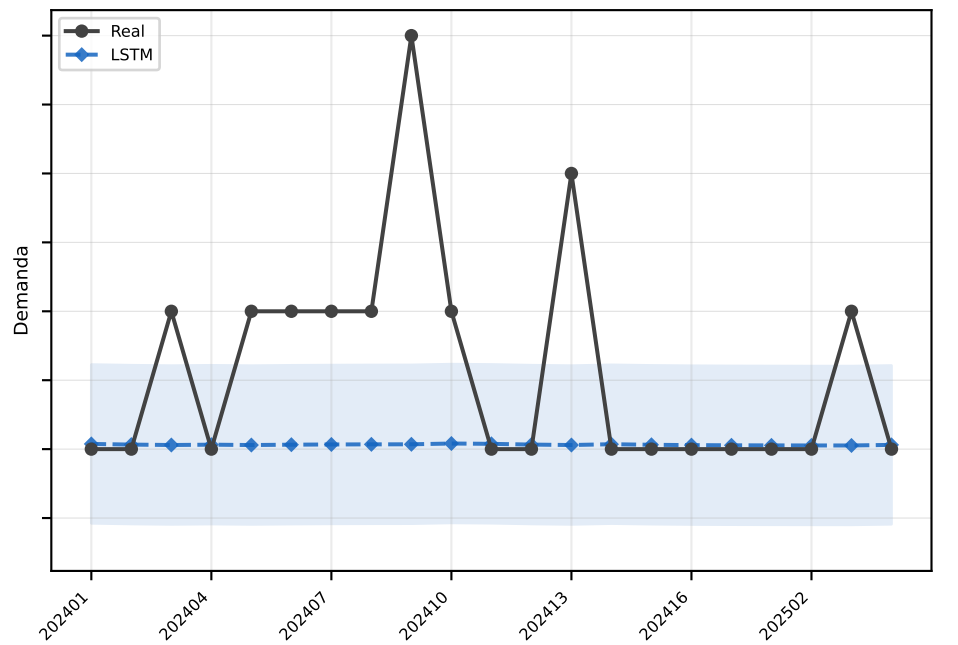
LSTM MAE=0.6
