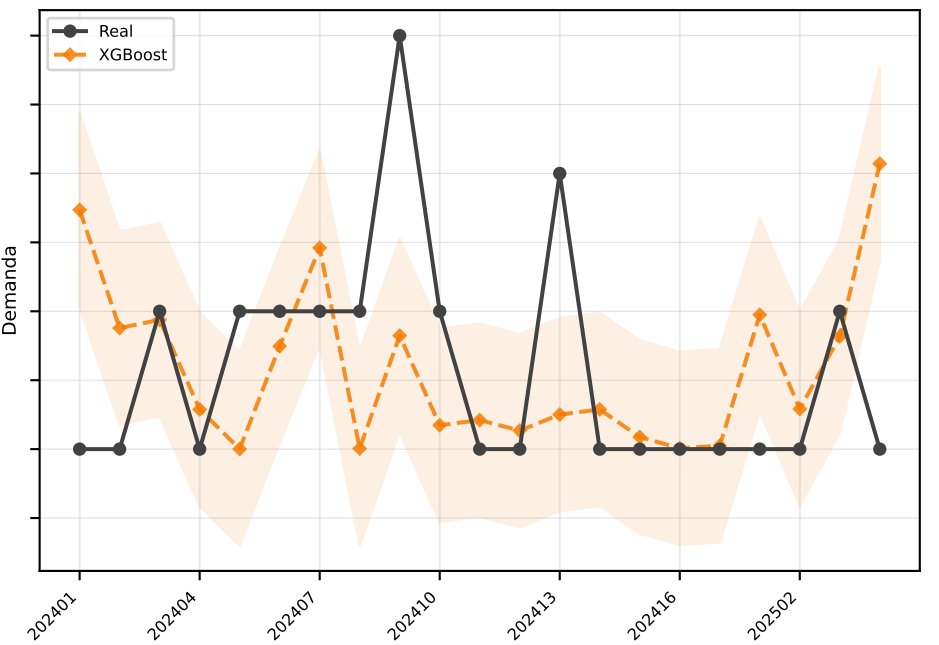
XGBoost MAE=0.7
