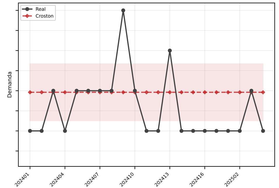
Croston MAE=0.7
