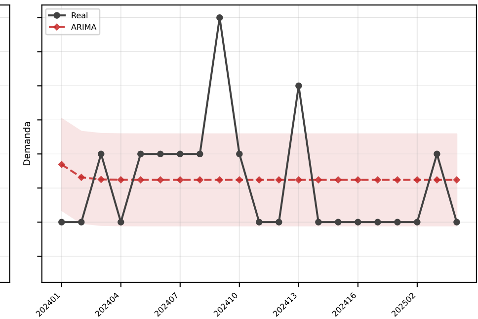
ARIMA MAE=0.7
