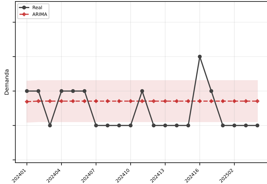
ARIMA MAE=0.6
