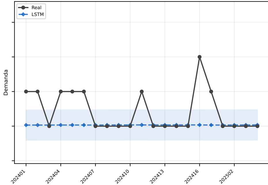
LSTM MAE=0.4
