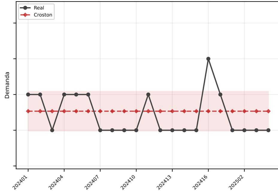
Croston MAE=0.6
