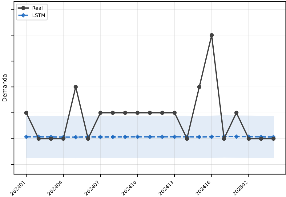
LSTM MAE=0.8
