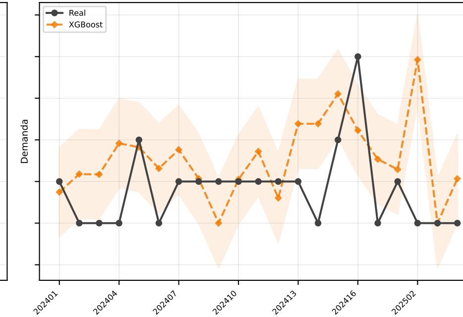
XGBoost MAE=1.1
