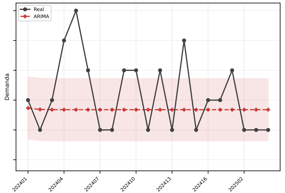
ARIMA MAE=1.0
