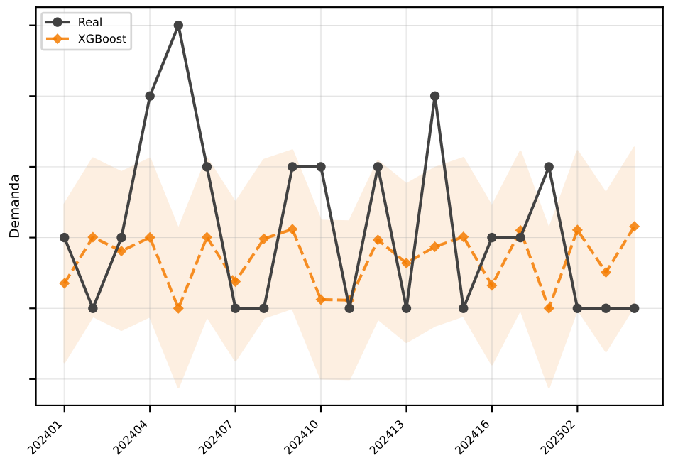
XGBoost MAE=1.1
