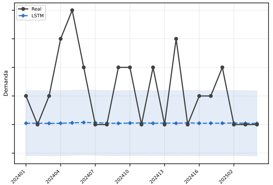
LSTM MAE=1.1
