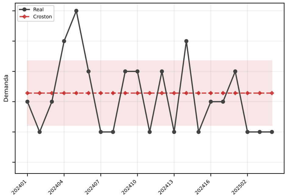
Croston MAE=1.1
