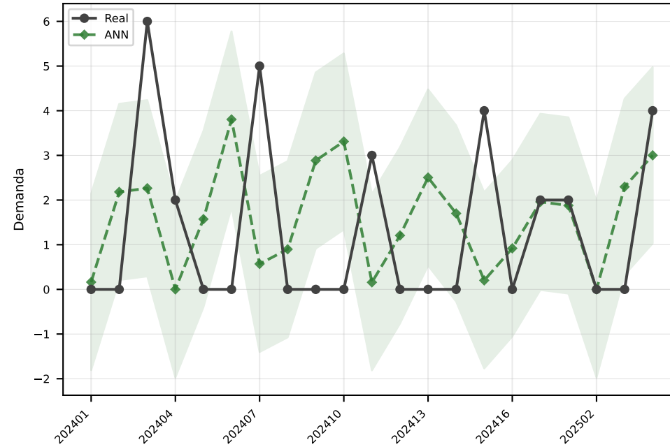
ANN MAE=2.0
