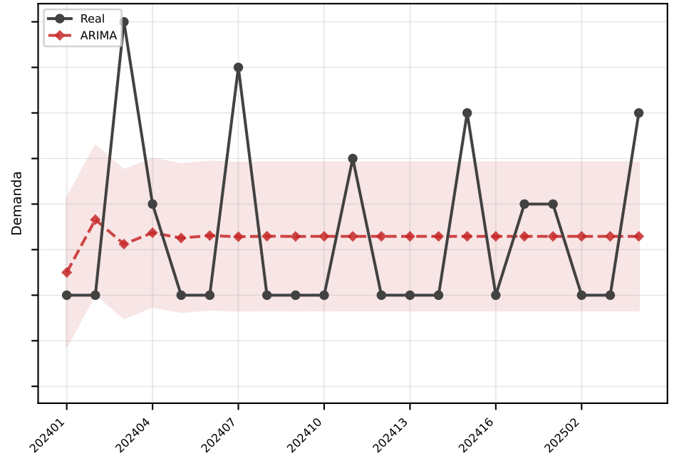
ARIMA MAE=1.6
