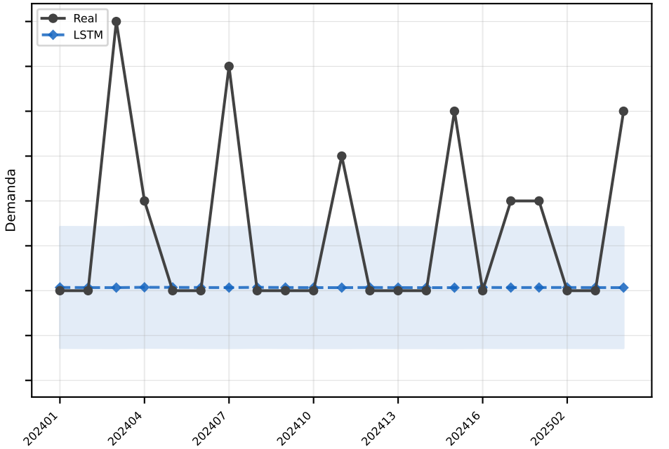
LSTM MAE=1.4
