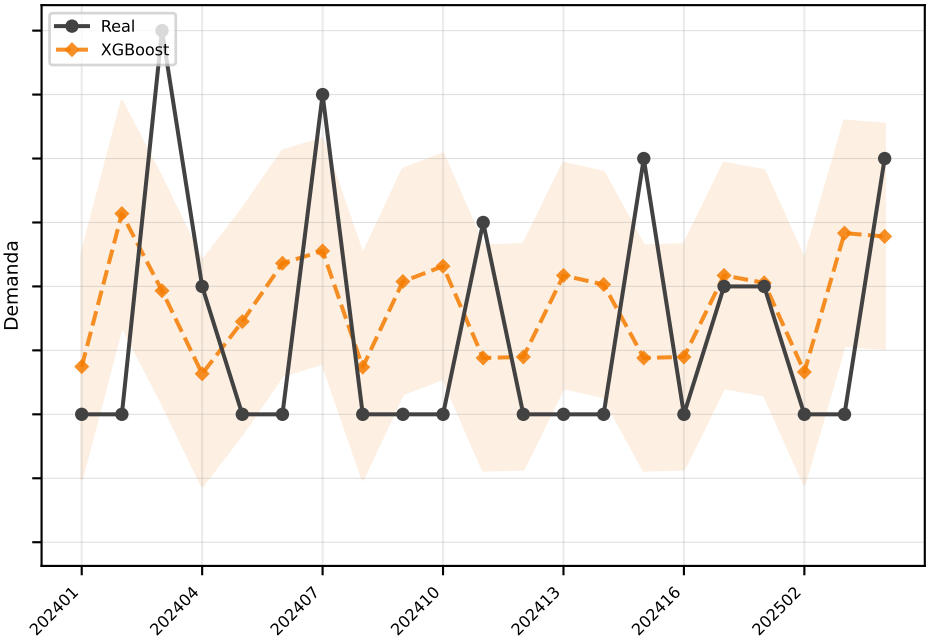
XGBoost MAE=1.8
