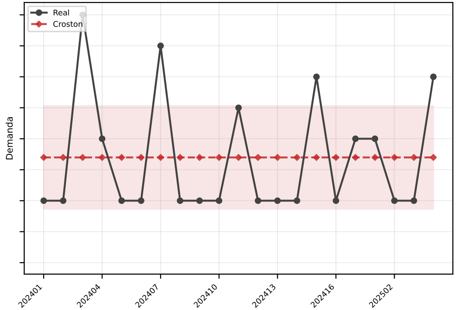
Croston MAE=1.7
