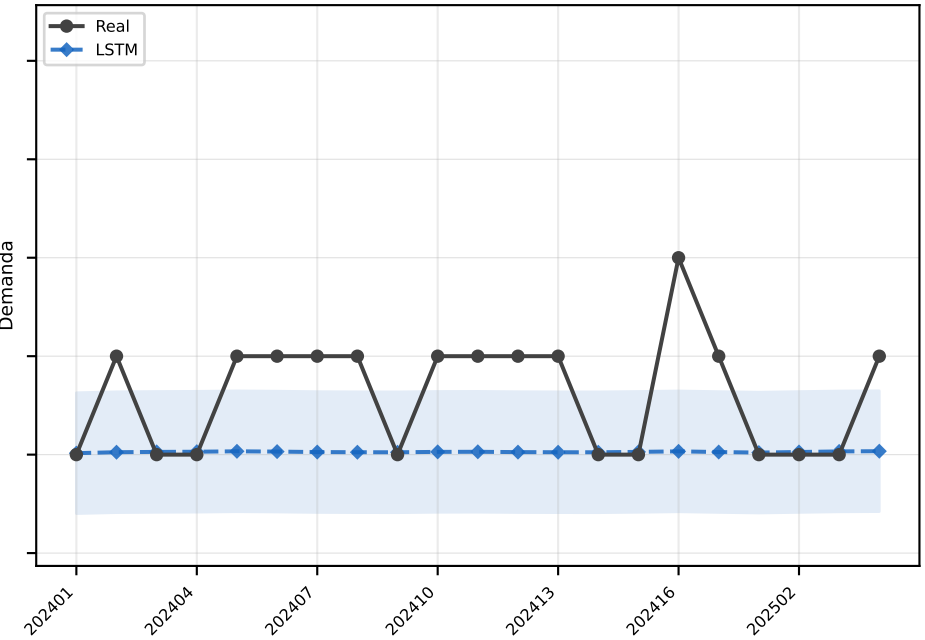
LSTM MAE=0.6
