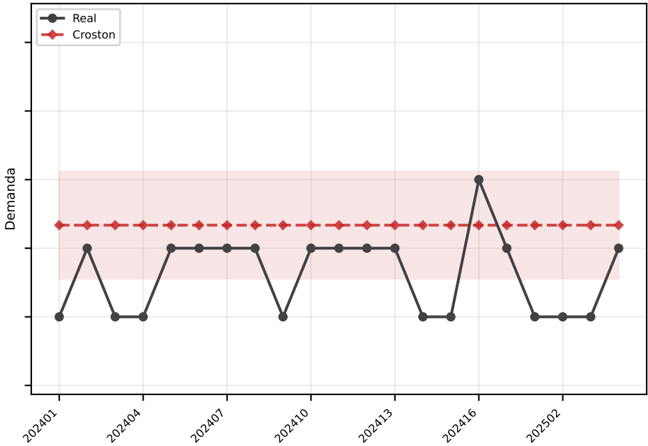
Croston MAE=0.8
