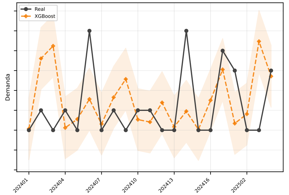
XGBoost MAE=1.6
