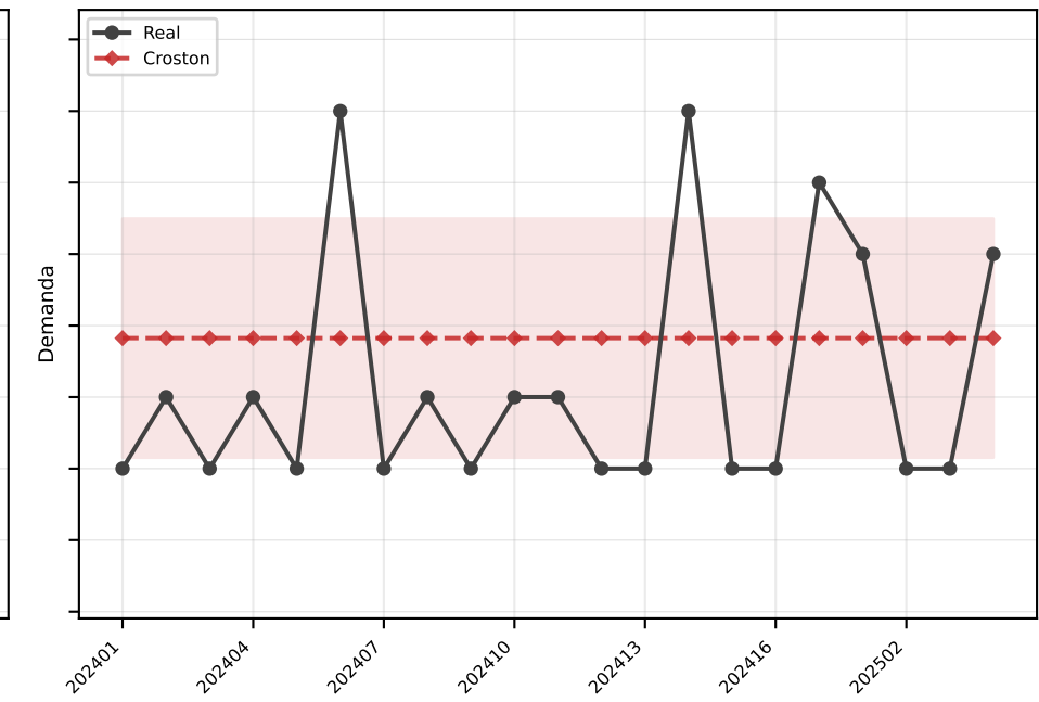
Croston MAE=1.7
