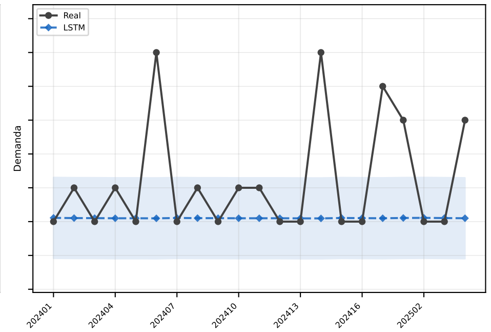
LSTM MAE=1.2
