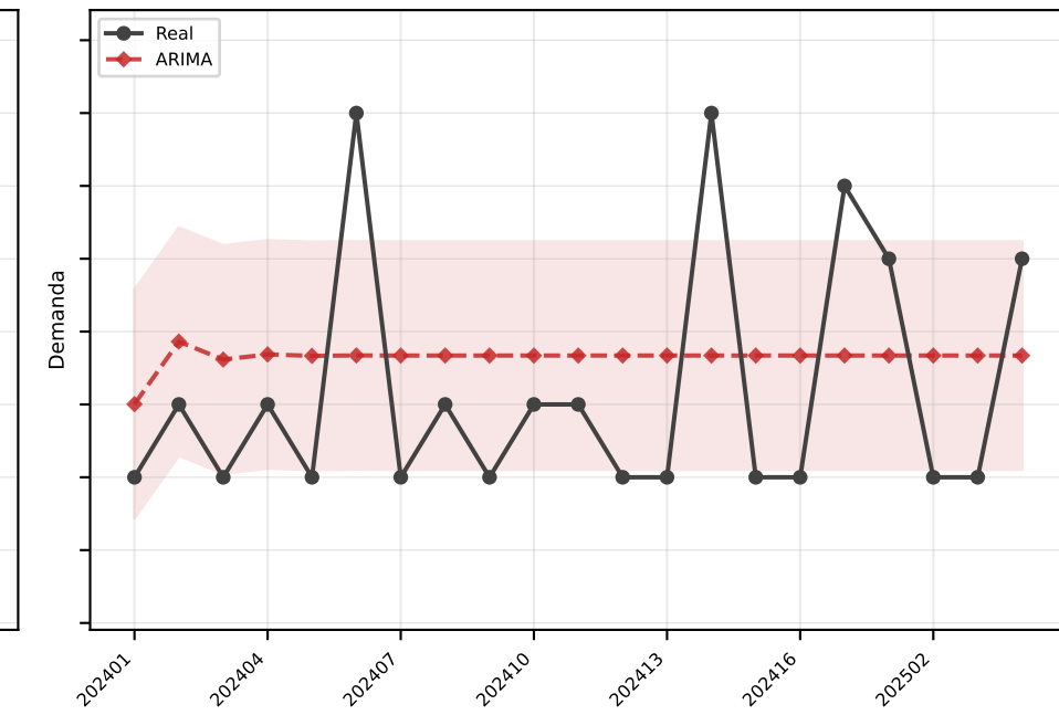
ARIMA MAE=1.6
