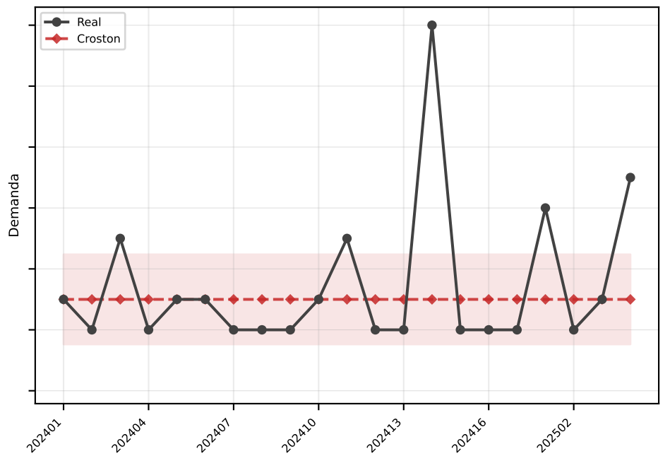
Croston MAE=1.5
