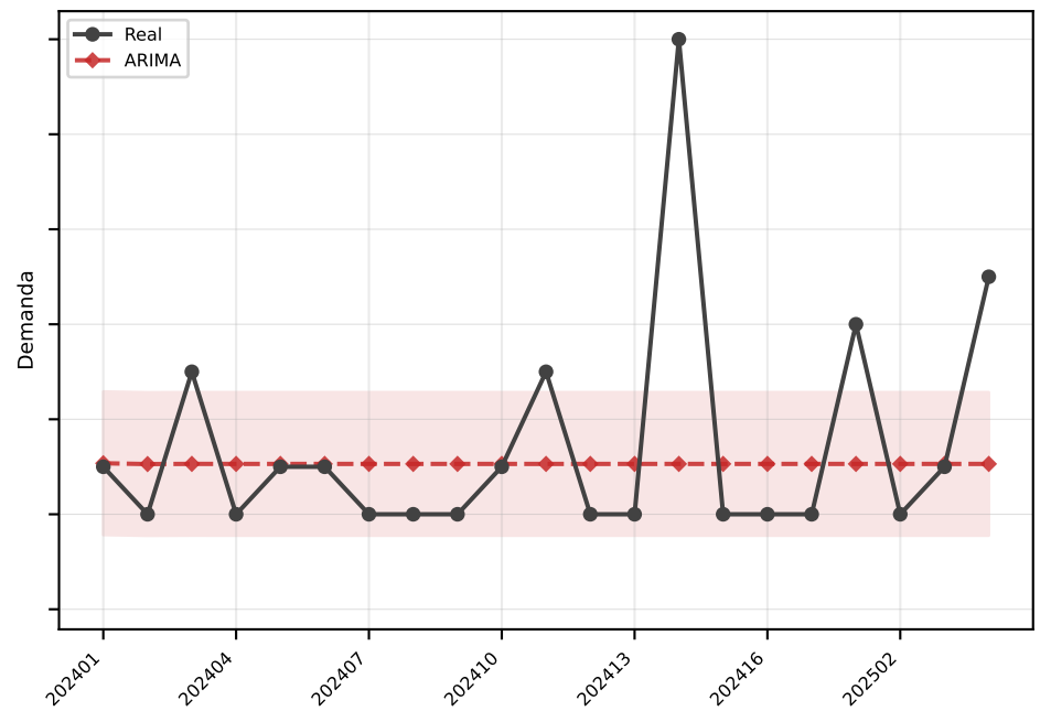
ARIMA MAE=1.5
