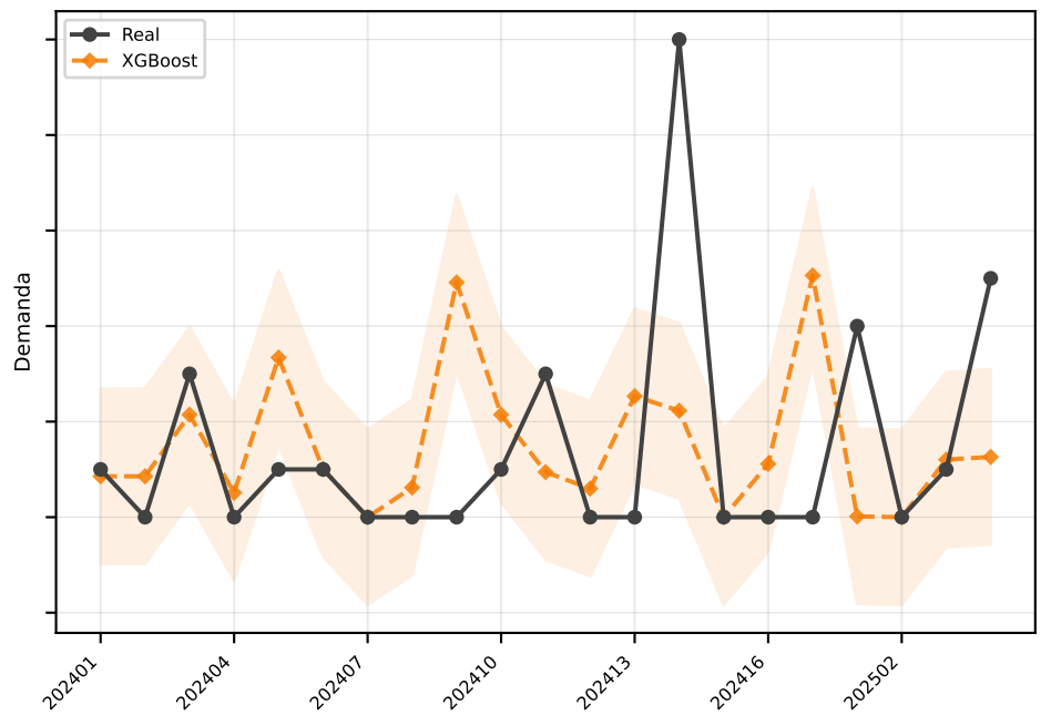
XGBoost MAE=1.8
