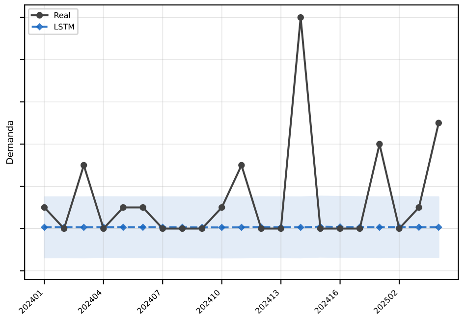
LSTM MAE=1.4
