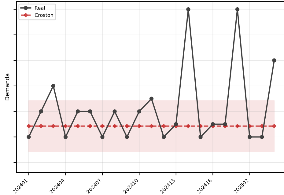
Croston MAE=2.0
