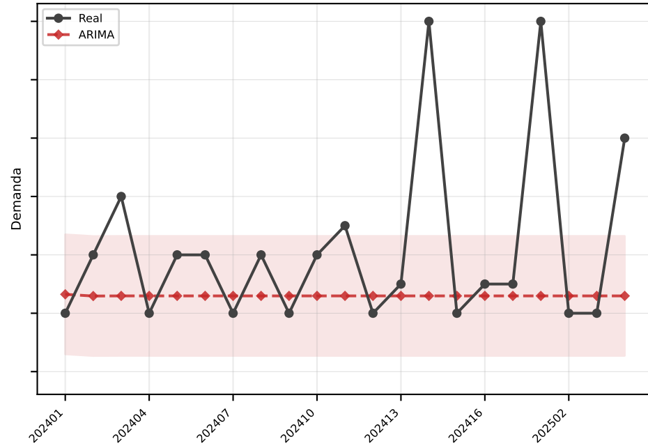
ARIMA MAE=2.1
