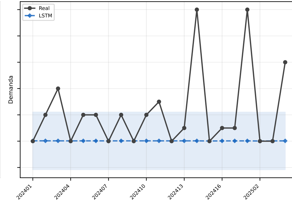
LSTM MAE=2.2
