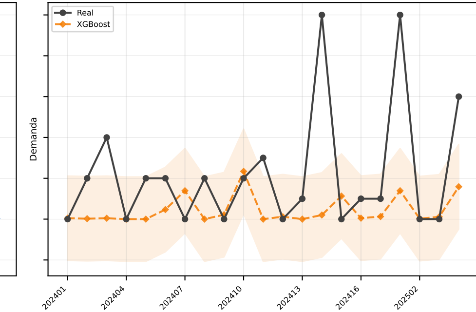
XGBoost MAE=2.1
