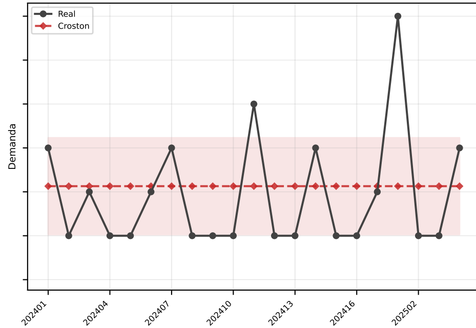
Croston MAE=1.1
