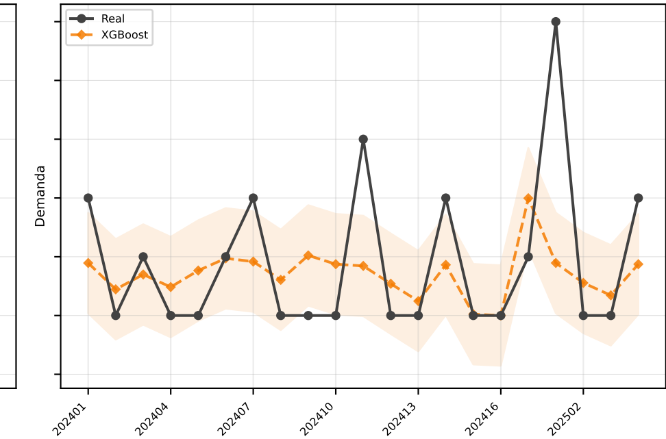
XGBoost MAE=0.9
