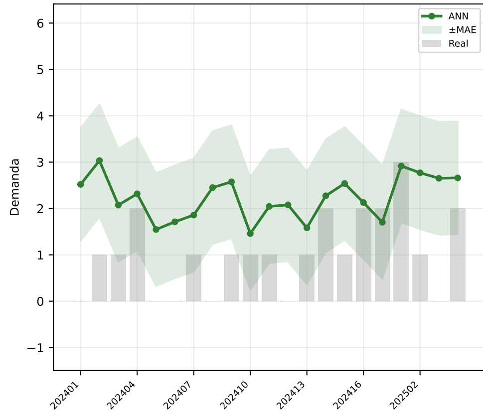
ANN (MAE = 1.2)
