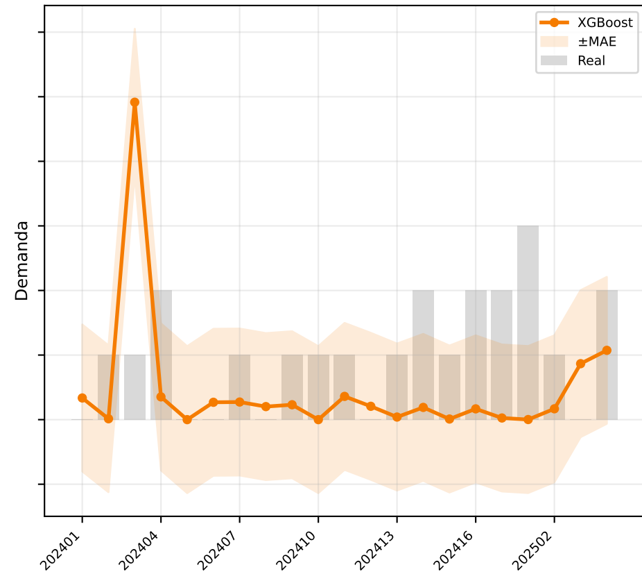
XGBoost (MAE = 1.1)
