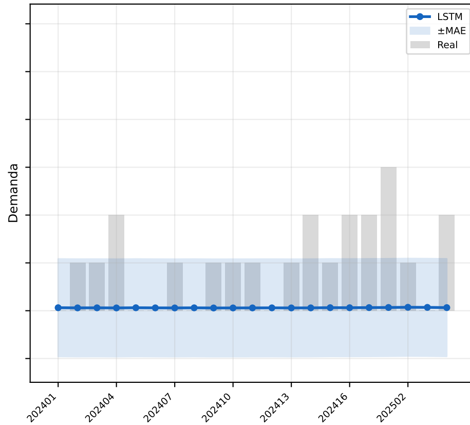
LSTM (MAE = 1.0)
