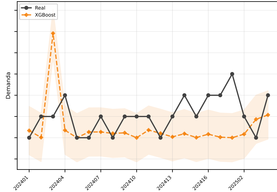
XGBoost MAE=1.1
