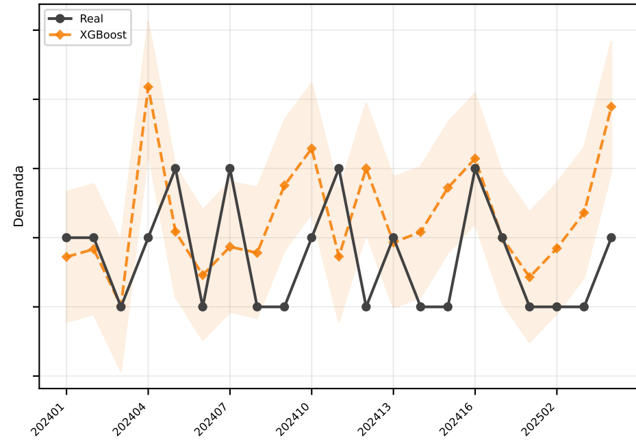
XGBoost MAE=0.9
