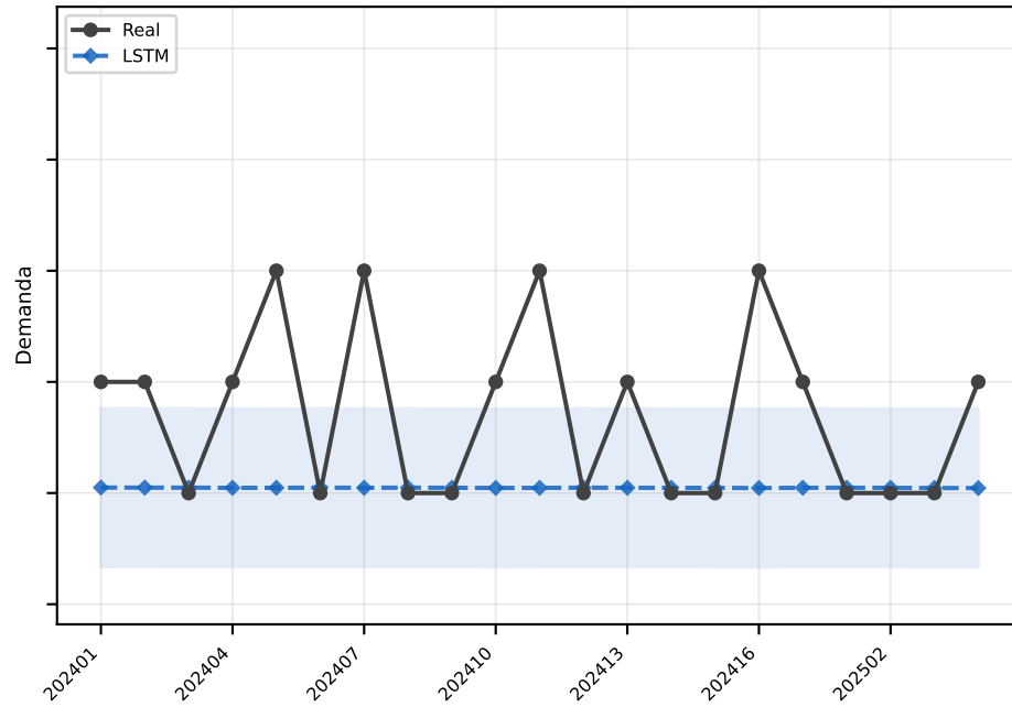
LSTM MAE=0.7
