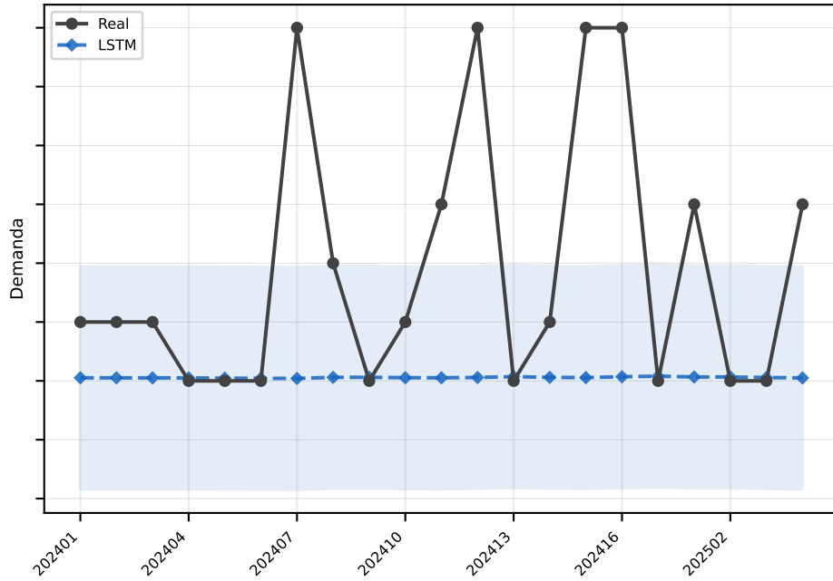
LSTM MAE=1.9
