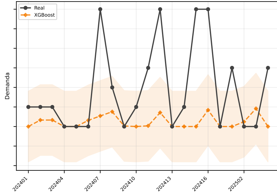
XGBoost MAE=1.8
