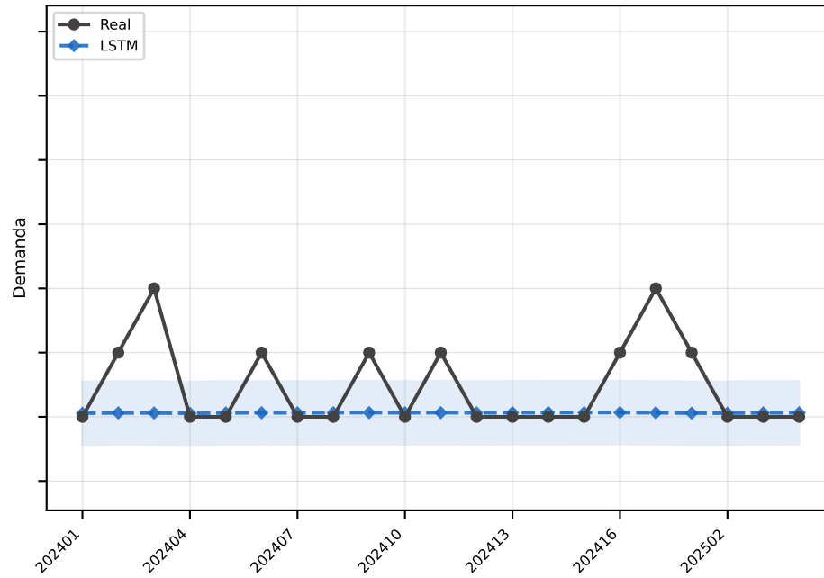
LSTM MAE=0.5
