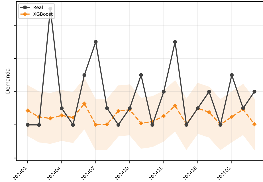
XGBoost MAE=1.5
