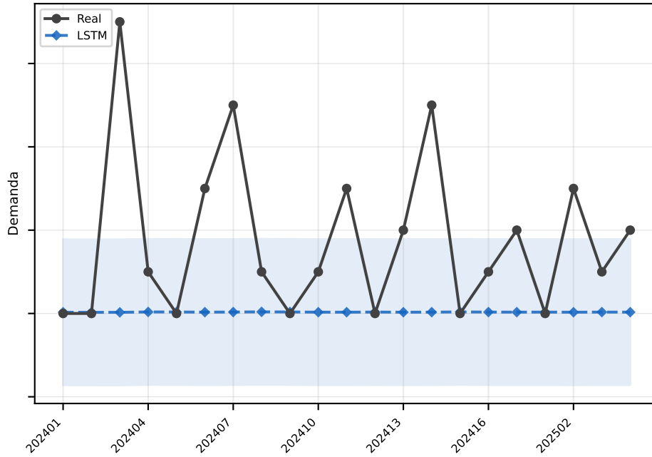
LSTM MAE=1.8
