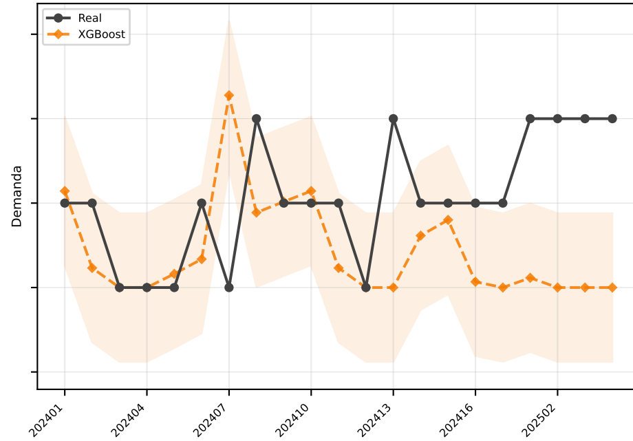
XGBoost MAE=0.9
