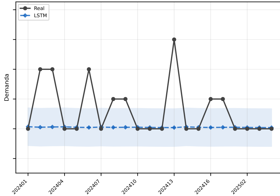
LSTM MAE=0.6
