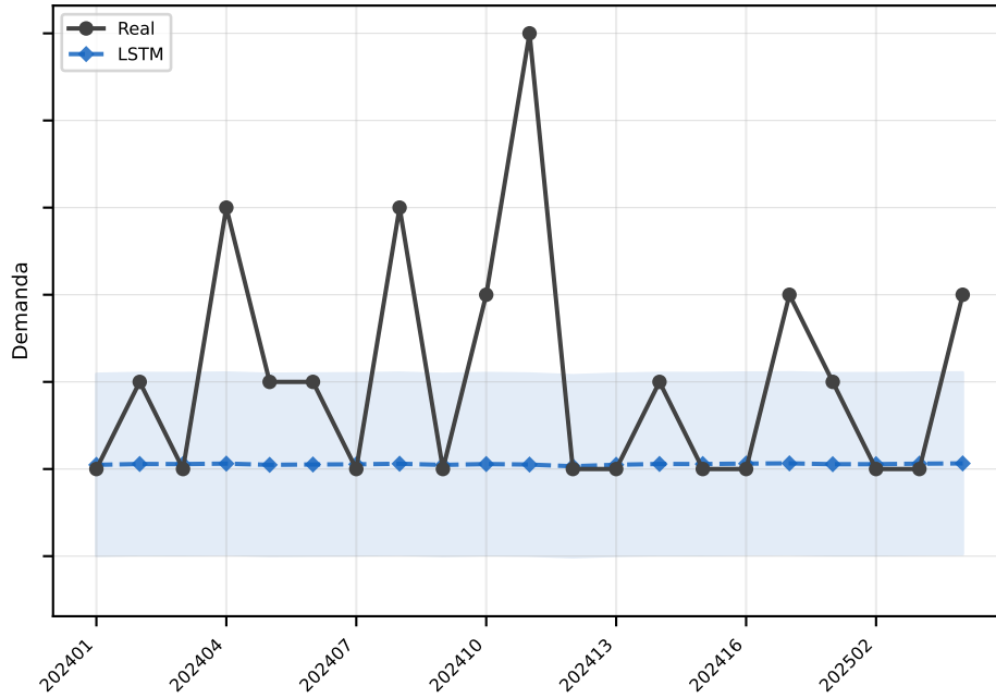
LSTM MAE=1.0
