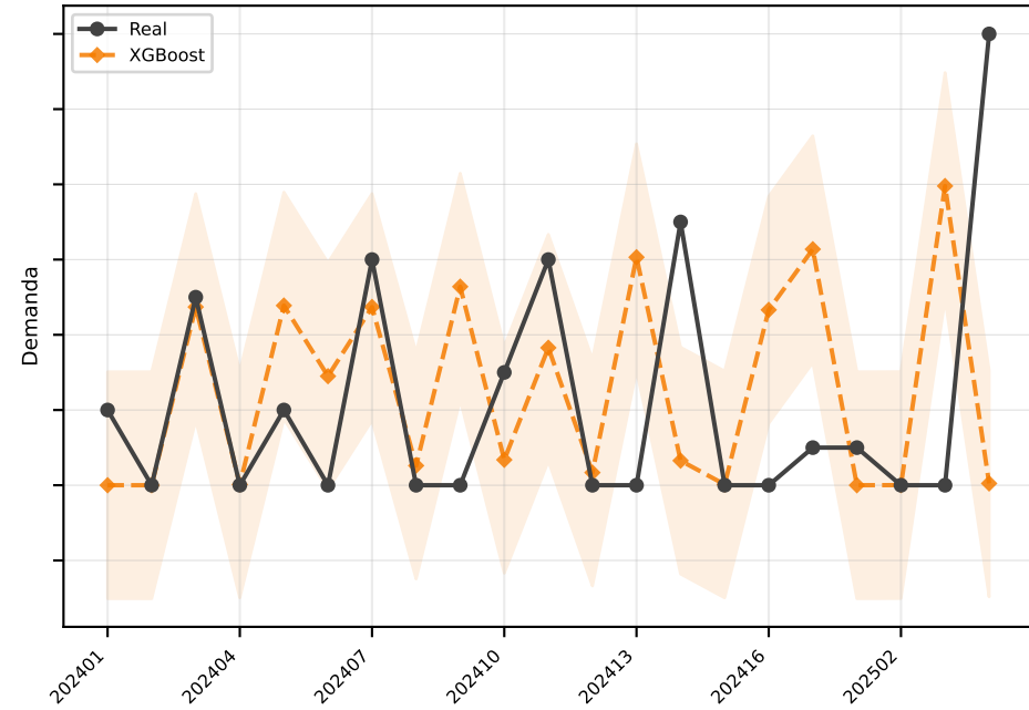
XGBoost MAE=3.0
