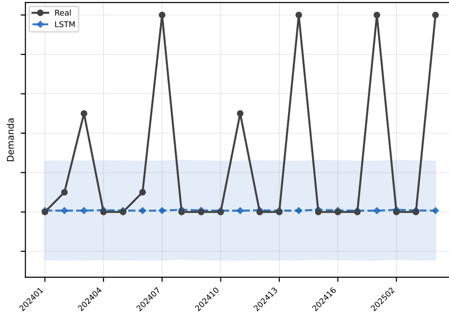
LSTM MAE=2.5
