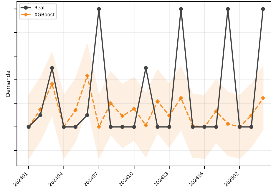
XGBoost MAE=2.7
