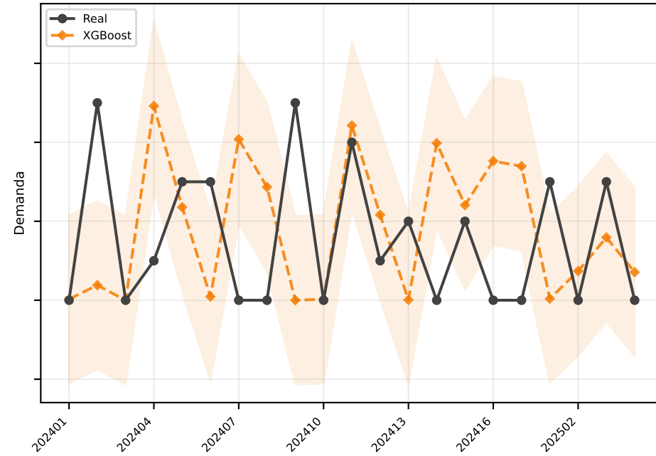
XGBoost MAE=2.1
