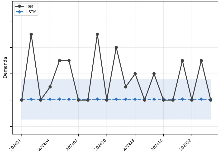
LSTM MAE=1.5
