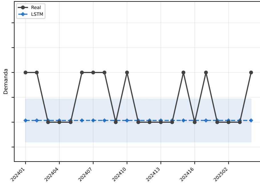
LSTM MAE=0.4
