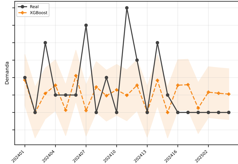
XGBoost MAE=1.5
