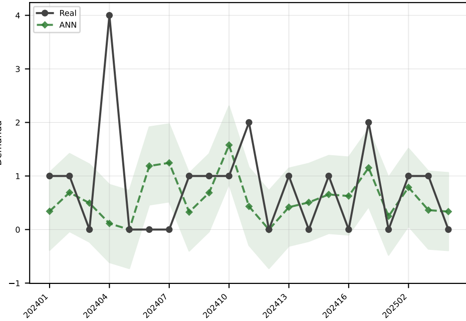
ANN MAE=0.7
