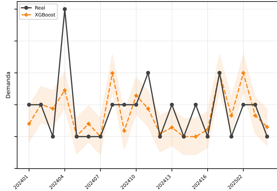
XGBoost MAE=0.6
