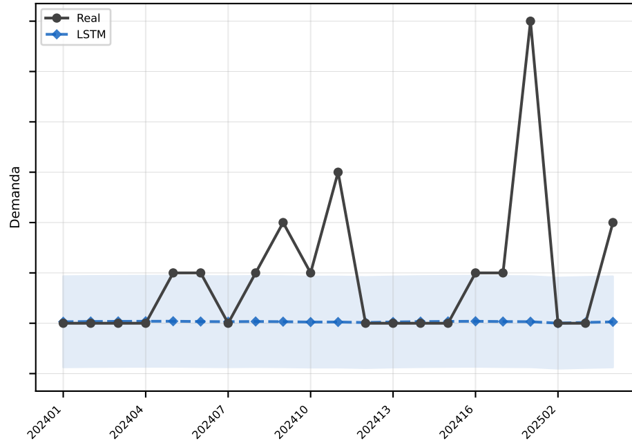
LSTM MAE=0.9
