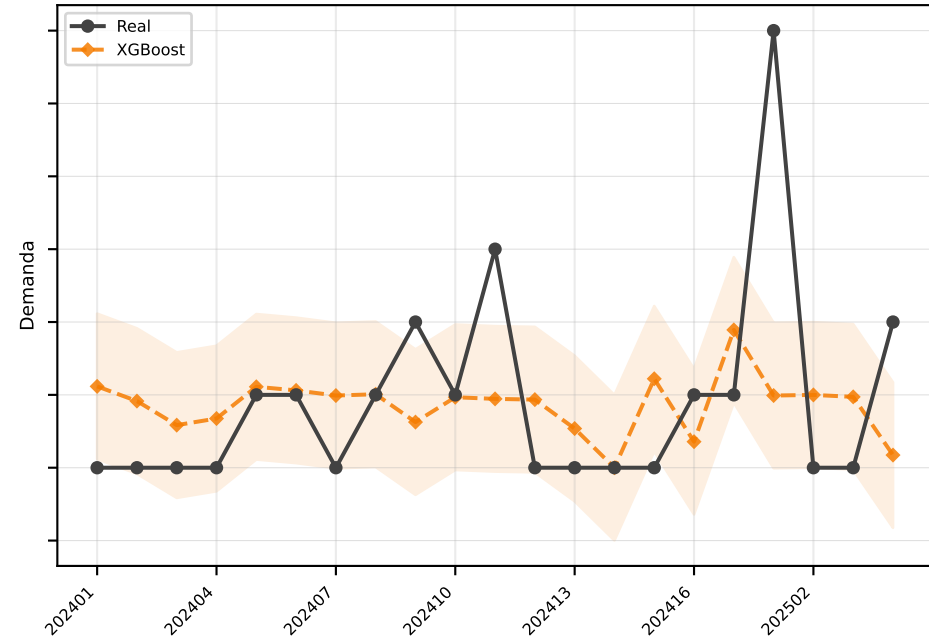
XGBoost MAE=1.0
