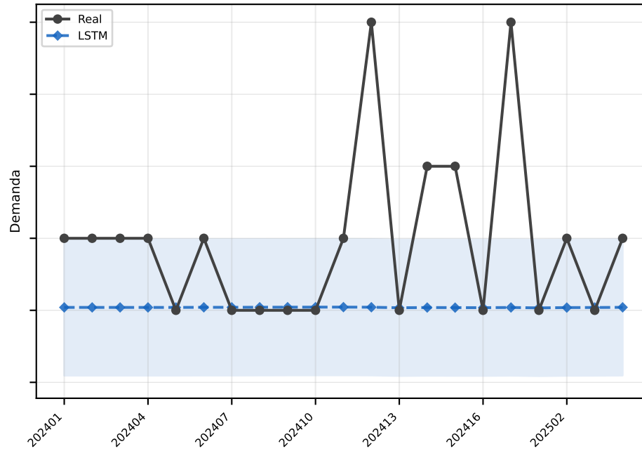
LSTM MAE=0.9
