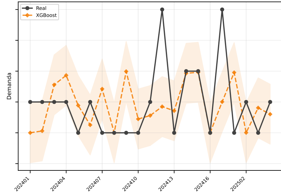
XGBoost MAE=1.0
