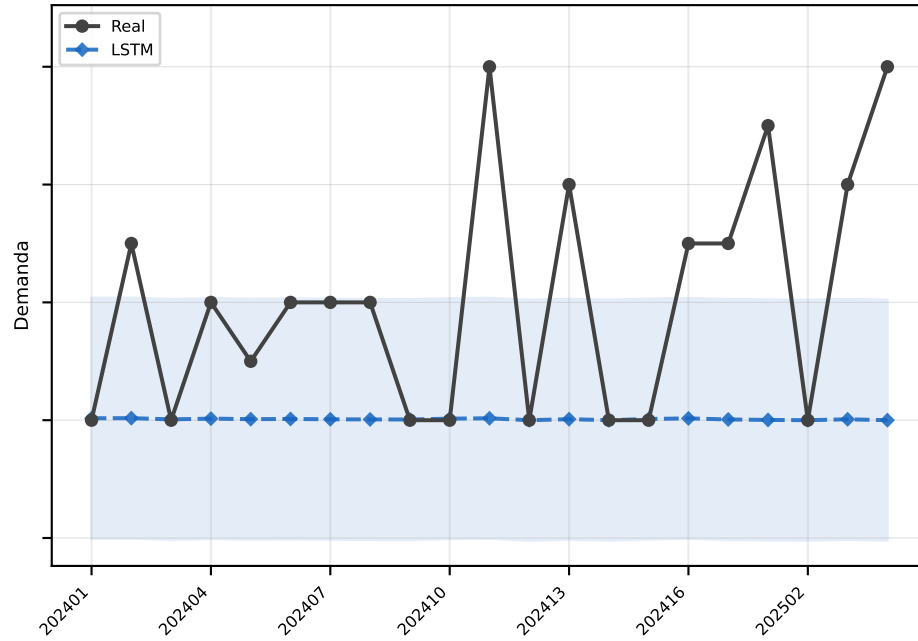
LSTM MAE=2.0
