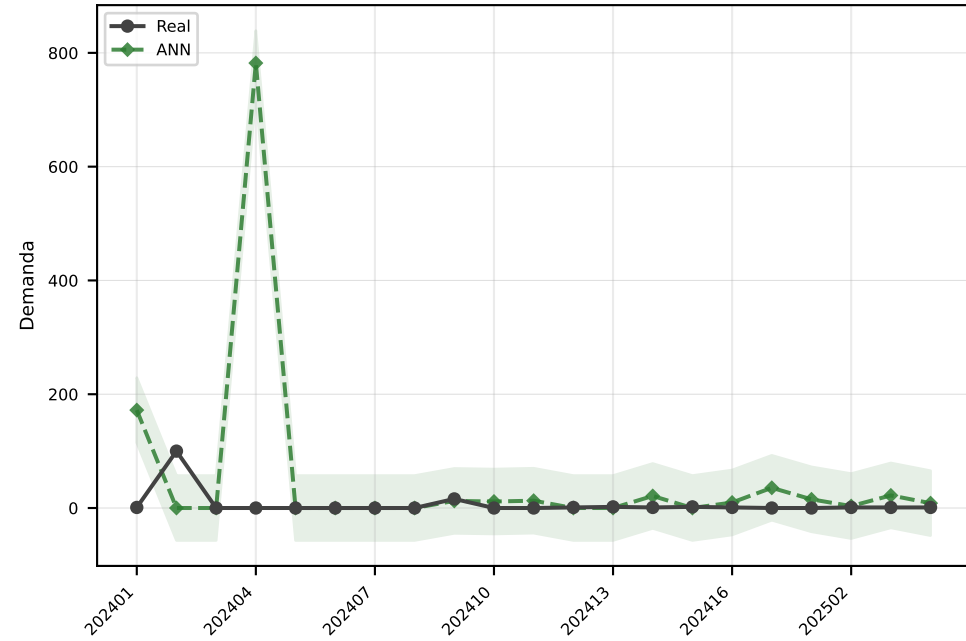
ANN MAE=57.0
