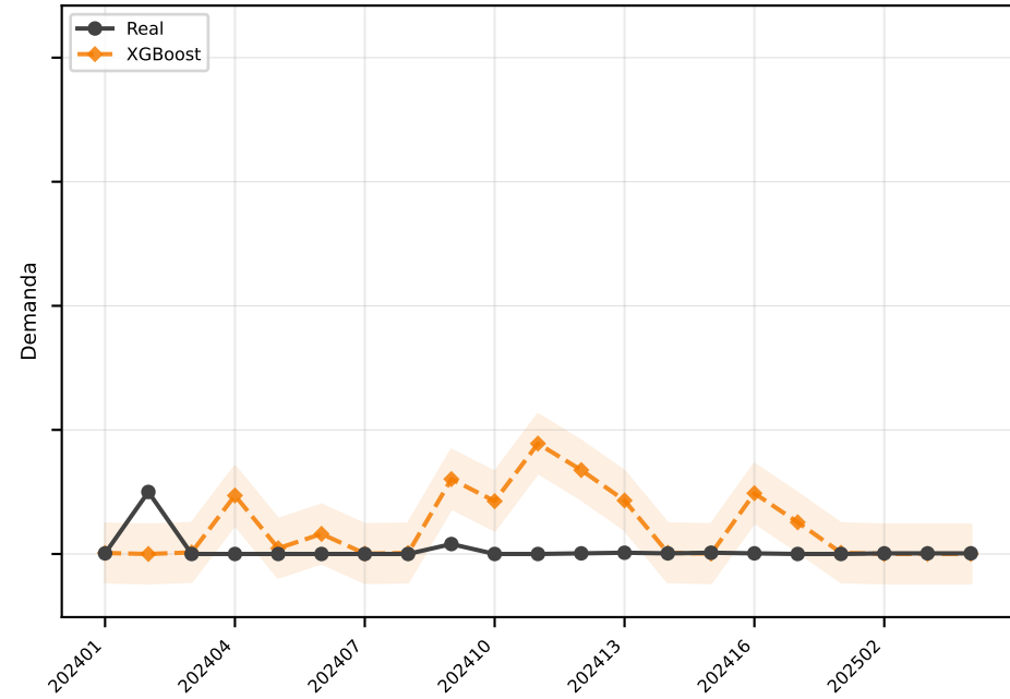
XGBoost MAE=46.8
