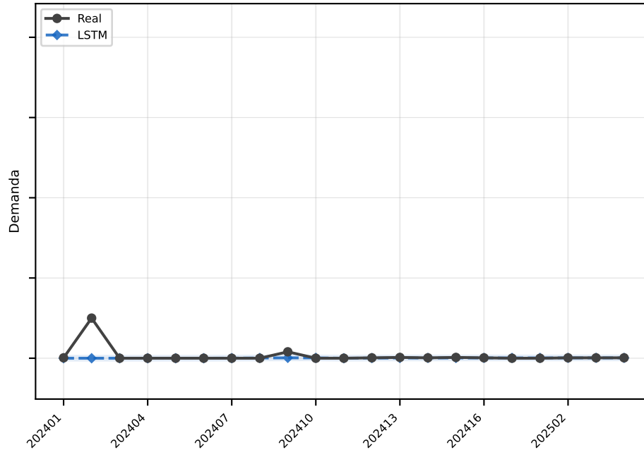
LSTM MAE=5.9
