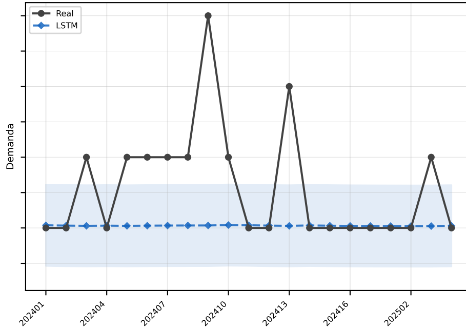
LSTM MAE=0.6
