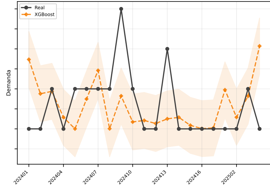
XGBoost MAE=0.7
