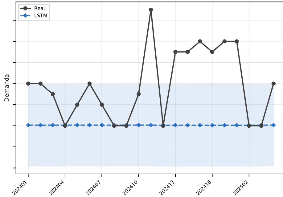
LSTM MAE=3.9
