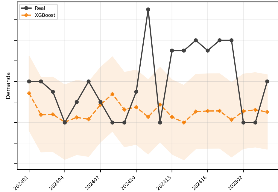
XGBoost MAE=3.6
