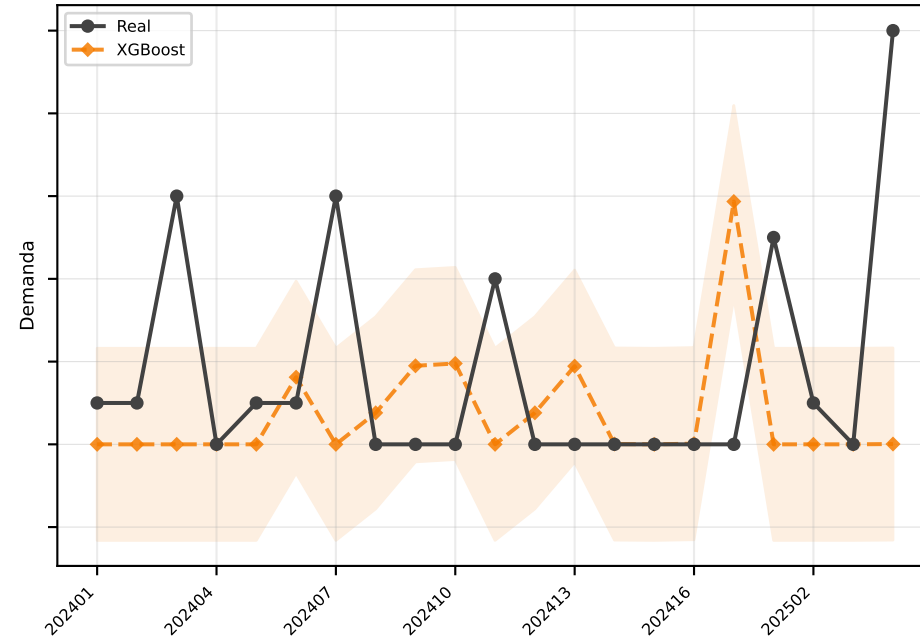
XGBoost MAE=2.3
