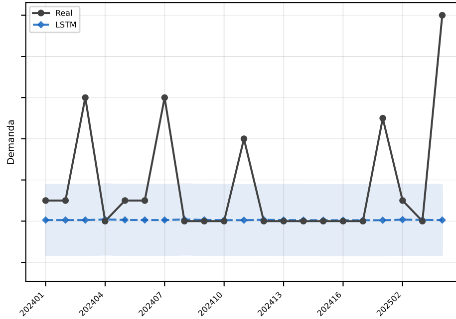
LSTM MAE=1.7
