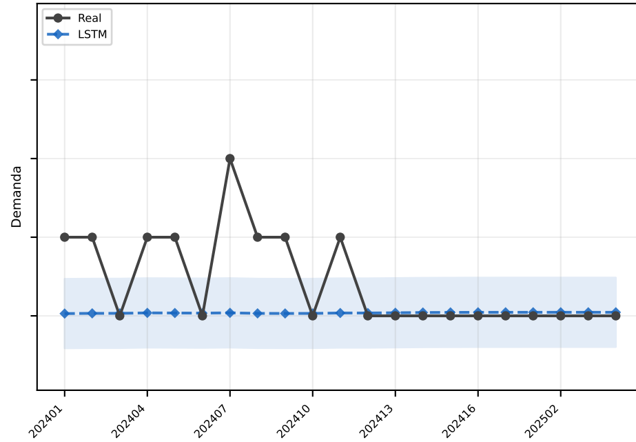
LSTM MAE=0.4
