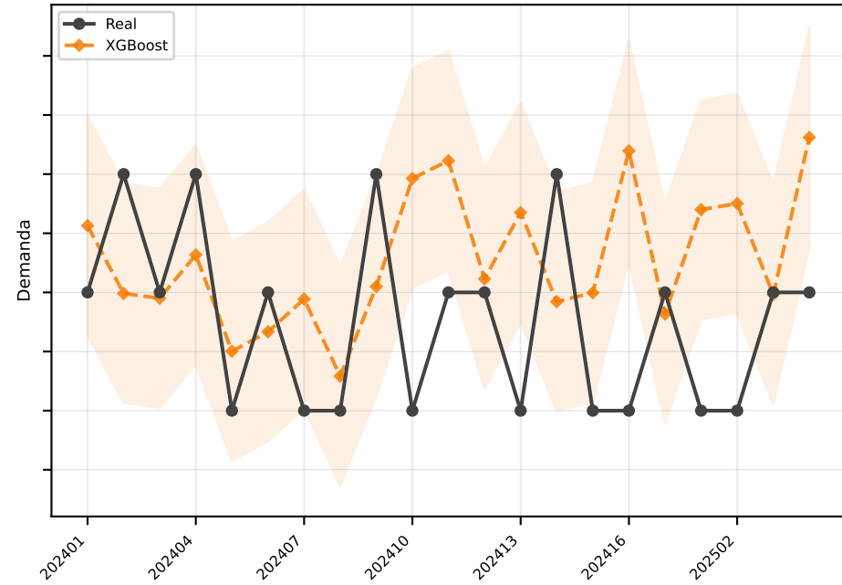
XGBoost MAE=0.9
