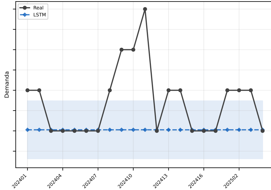
LSTM MAE=0.7
