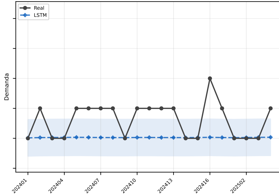
LSTM MAE=0.6
