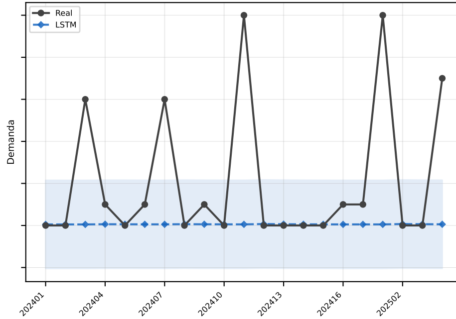
LSTM MAE=2.1
