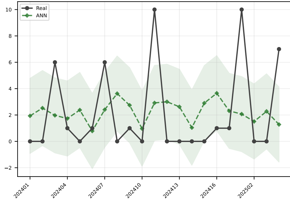
ANN MAE=2.8
