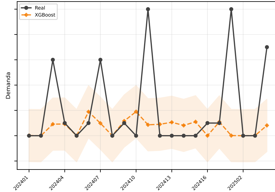
XGBoost MAE=2.1
